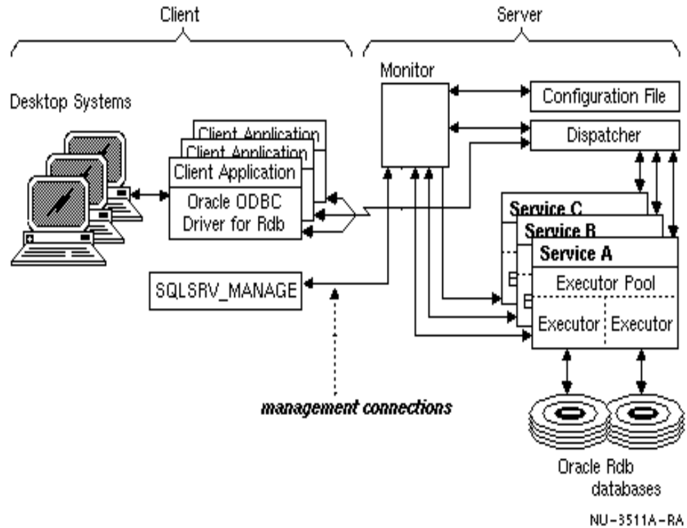
Figure 1-2 Oracle SQL/Services Architecture
