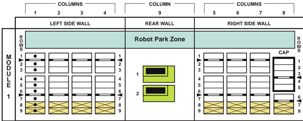
FIGURE A-1 Base Module Slots
