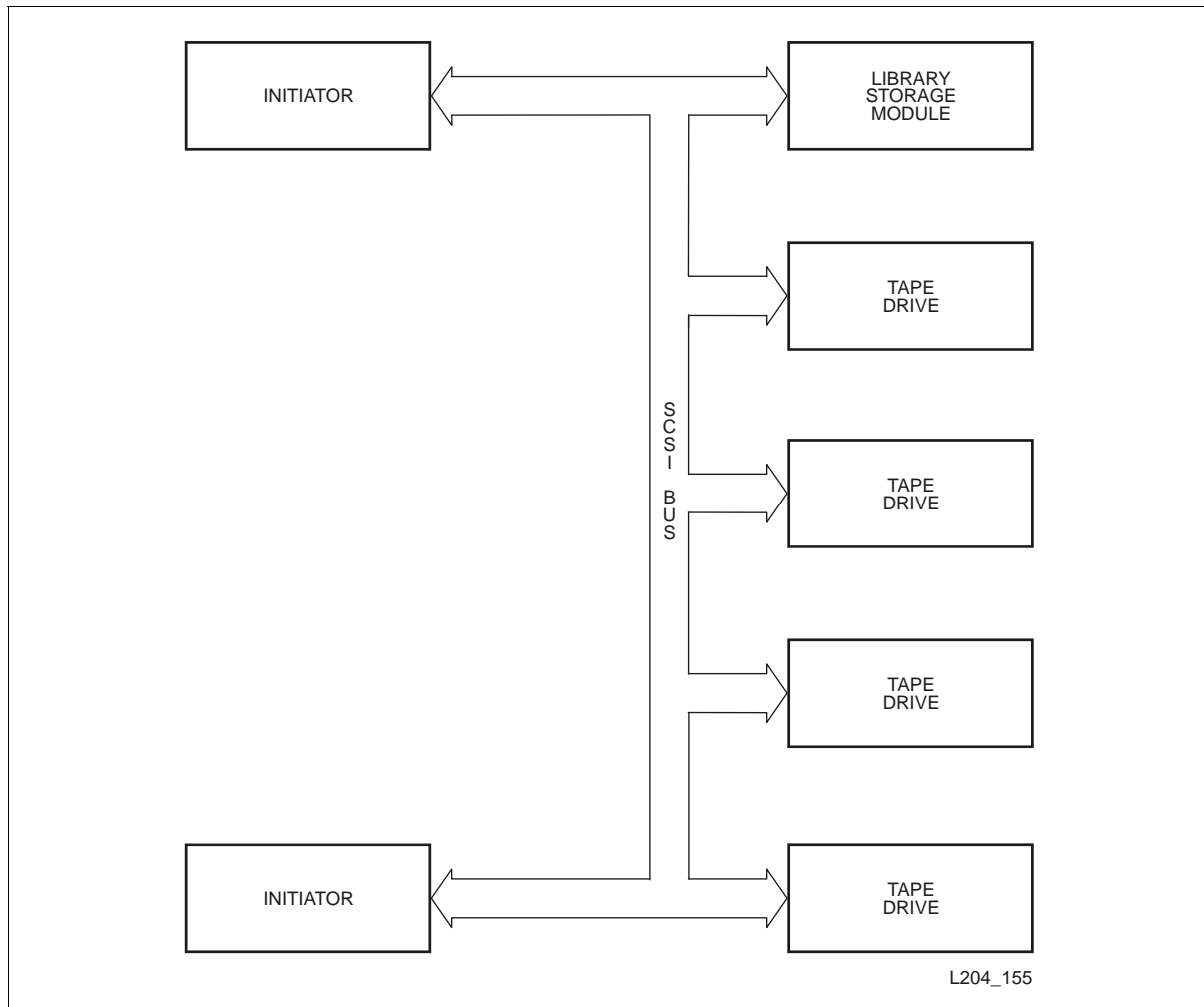
FIGURE 1-1 Example of a Library Configuration on the SCSI Bus
