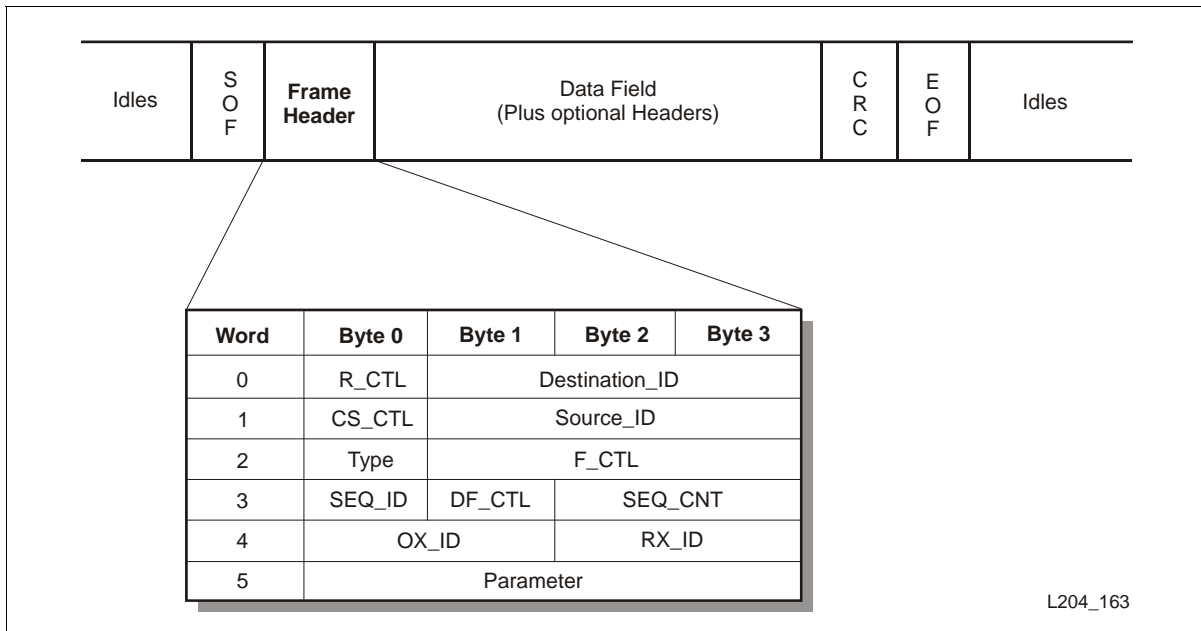
FIGURE 5-1 Frame and Frame Header Format
