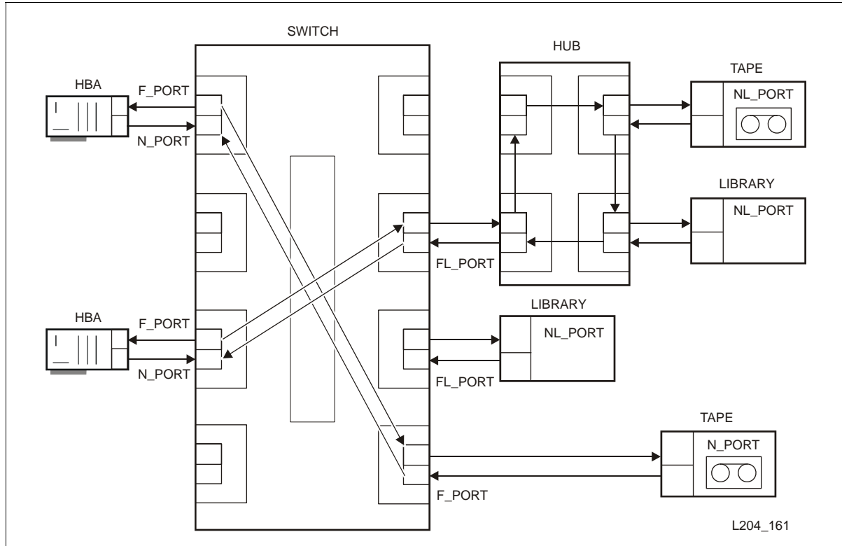
FIGURE 4-3 A Loop with a Hub Attached to a Switch
