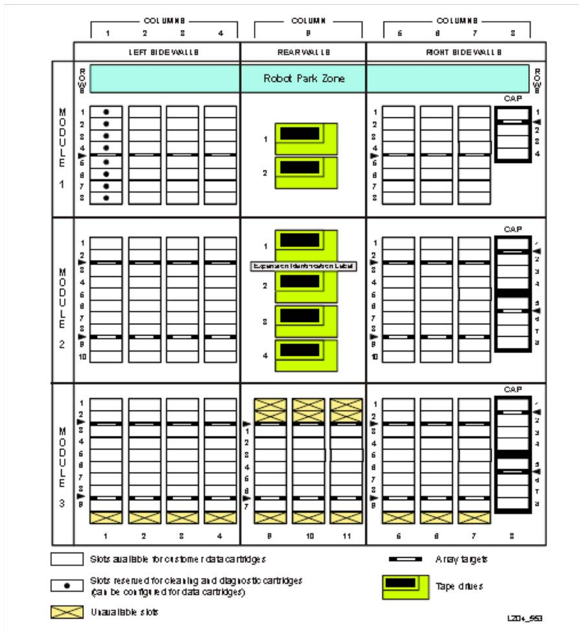
FIGURE 0-1 Partitioning a Library
