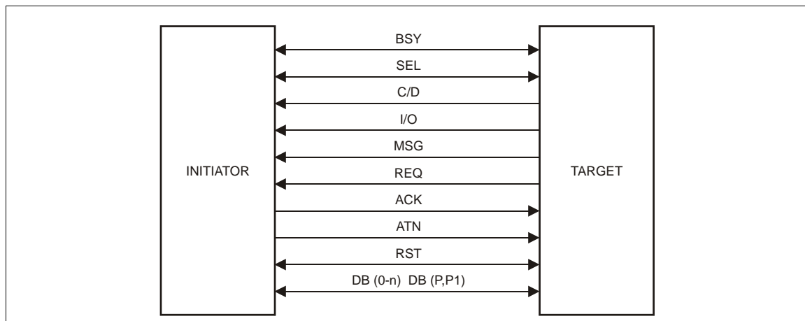
FIGURE 3-2 Signal Source and Direction
