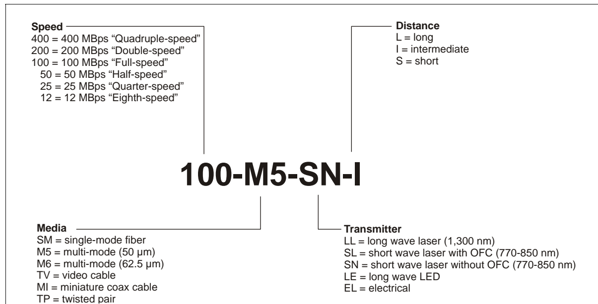
FIGURE 4-4 FC-0 Level Communication About Media (Cables)
