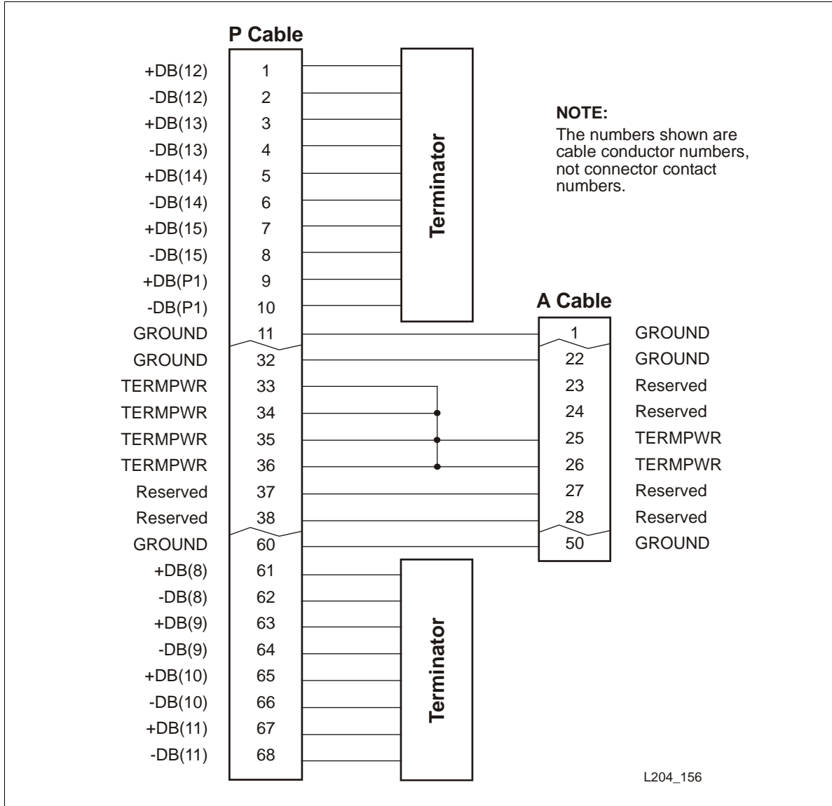
FIGURE 2-1 A-cable to P-cable Adapter
