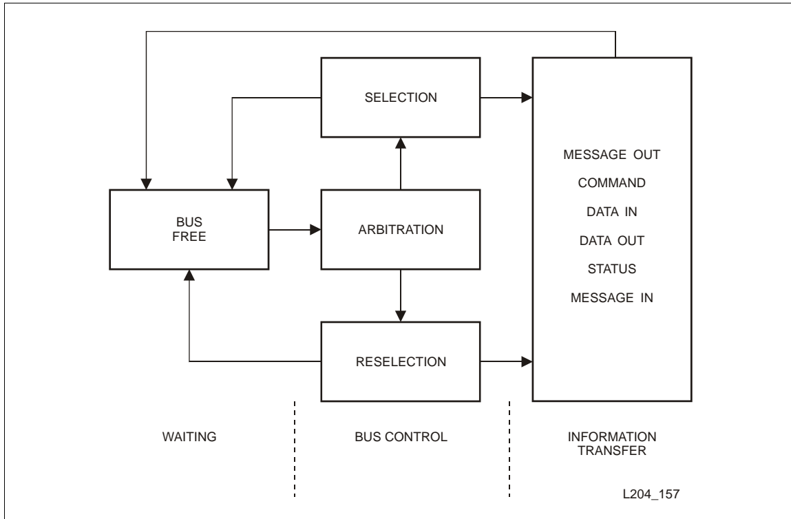
FIGURE 3-1 SCSI Bus Phases
