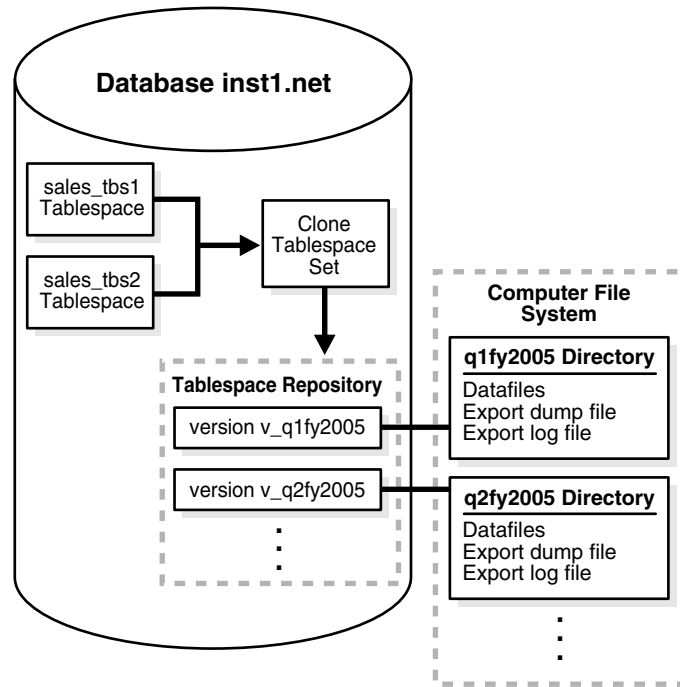
Figure 16–1 Example Tablespace Repository
