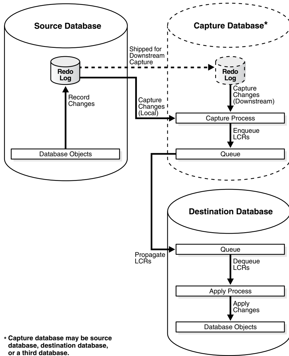
Figure B-1 Online Database Upgrade with Streams
