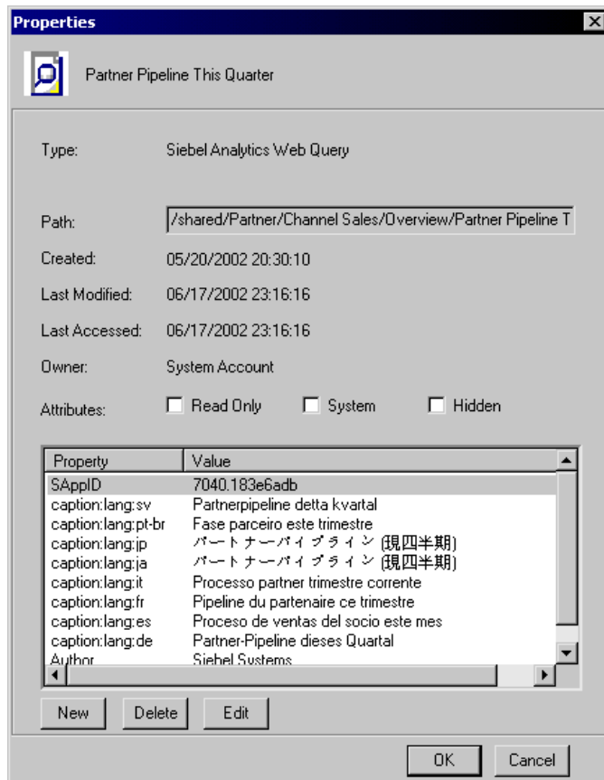
Figure 2. Properties Window
