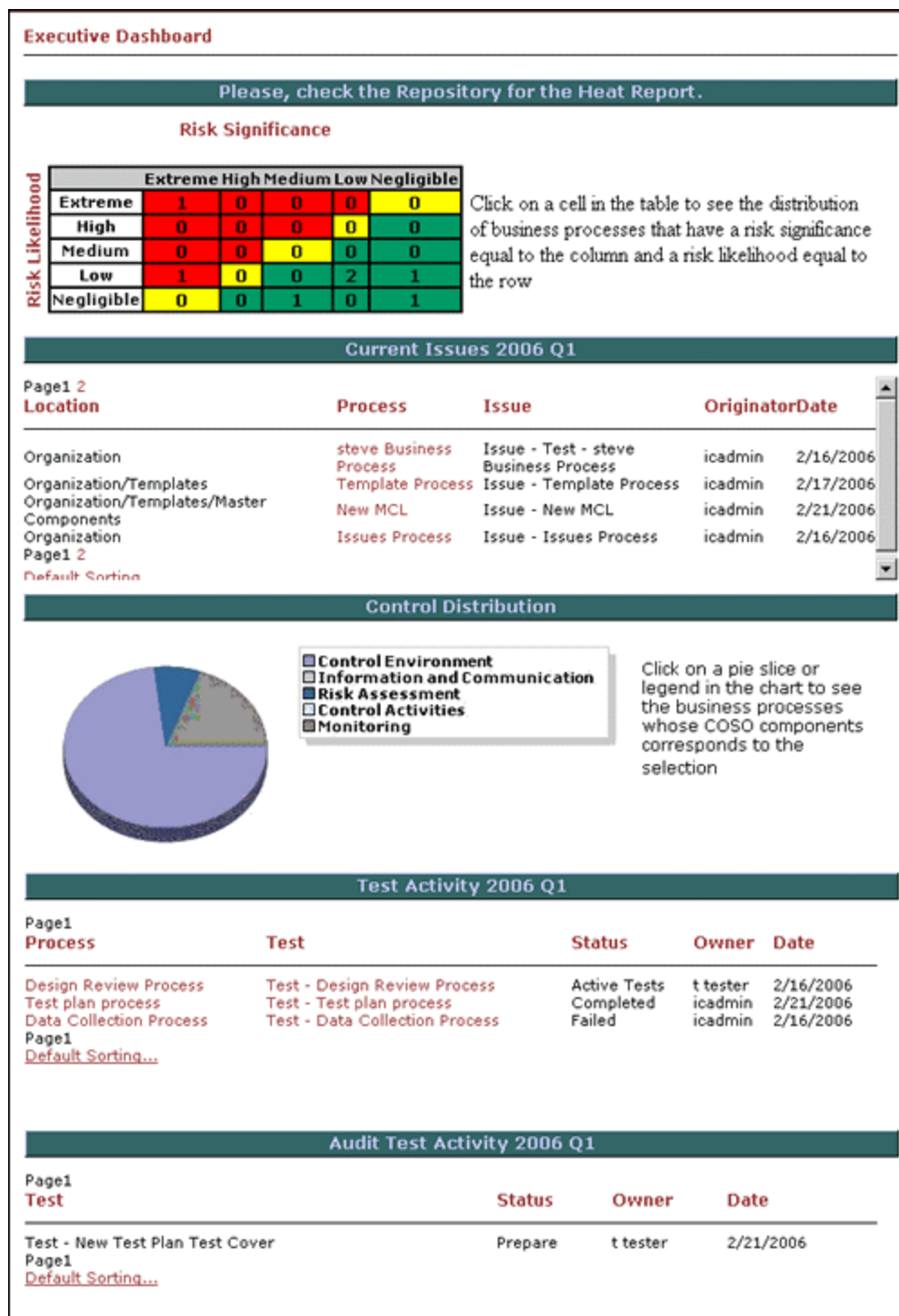
Figure 13-1 Executive Dashboard
