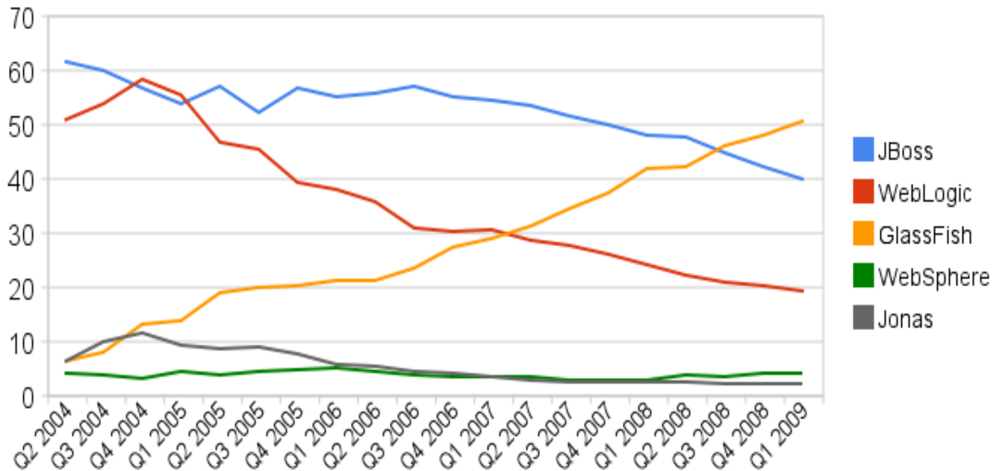
Java Deployment Descriptors, as % of Projects with Deployment Descriptors
