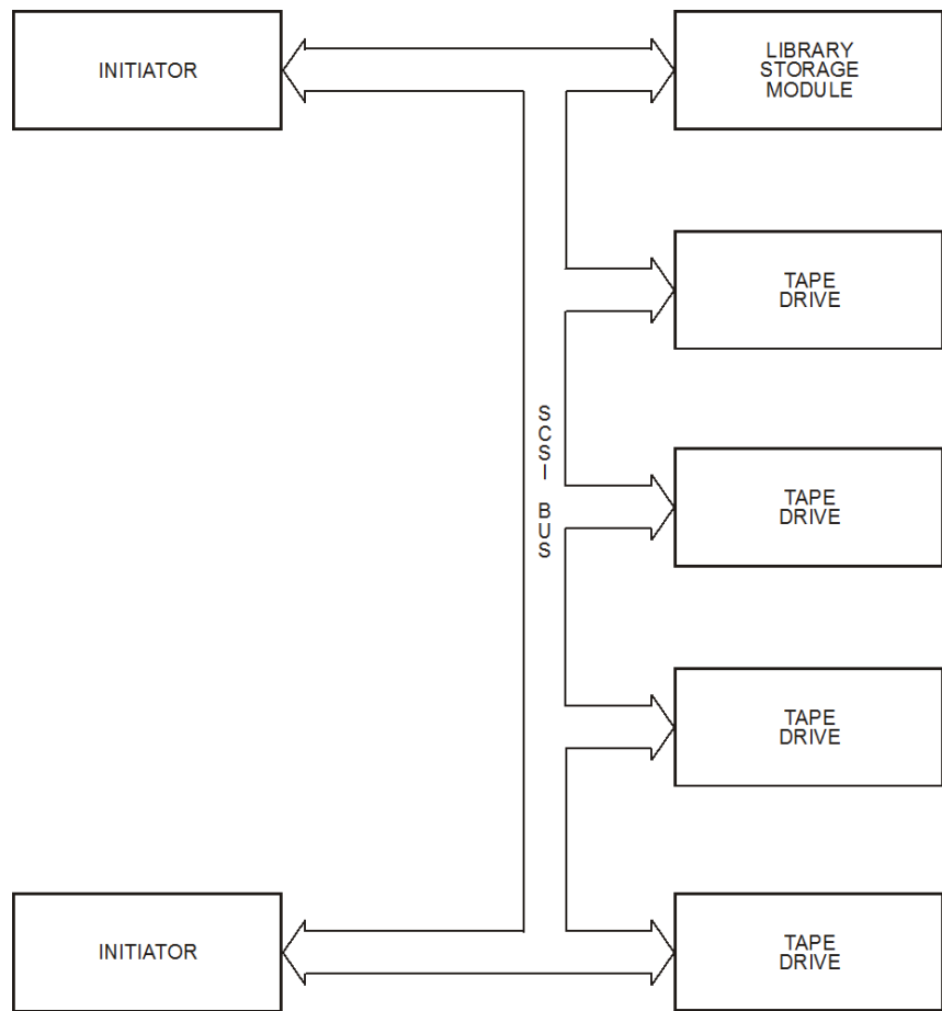
FIGURE 1-1 Example of a Library Configuration on the SCSI Bus
