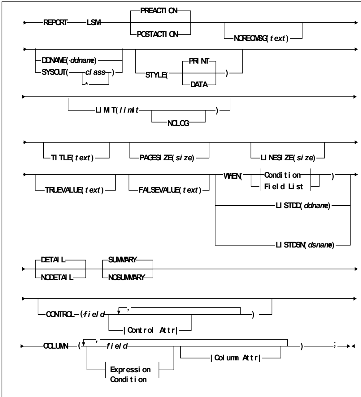
FIGURE 6-35 REPORT LSM Statement Syntax - Part 1
