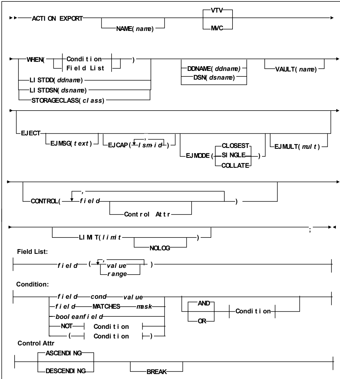
FIGURE 5-4 ACTION EXPORT Statement Syntax
