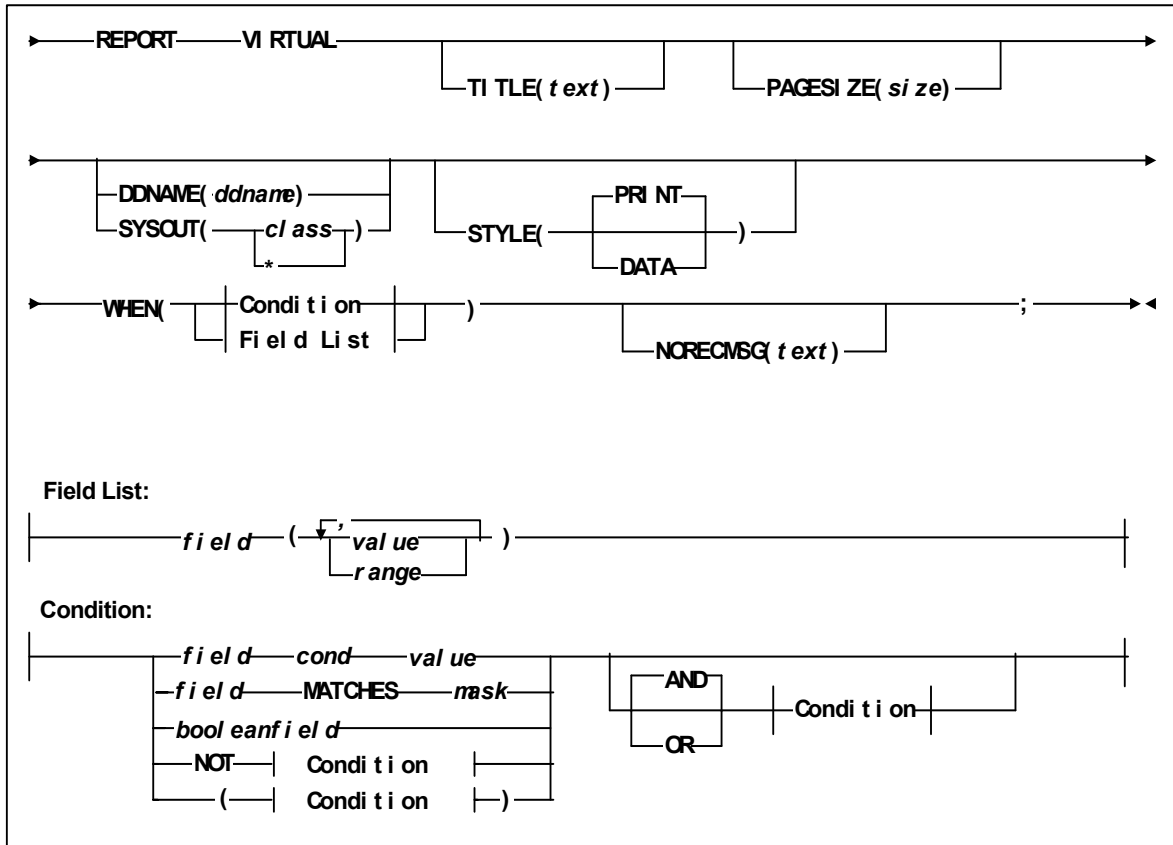
FIGURE 6-34 REPORT VIRTUAL Statement Syntax
