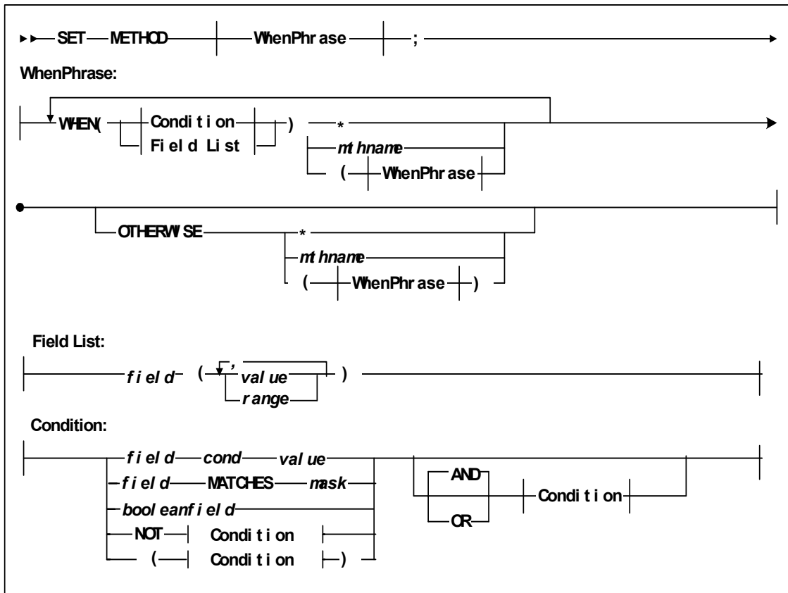
FIGURE 4-12 SET METHOD Statement Syntax
