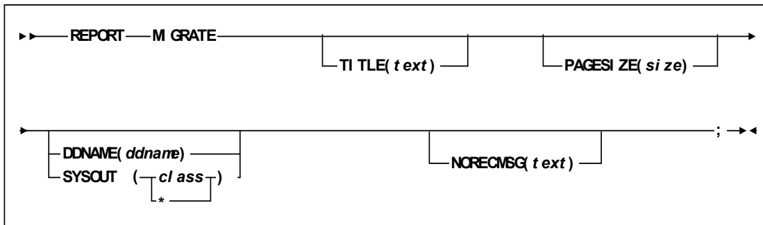
FIGURE 6-11 REPORT MIGRATE Statement Syntax
