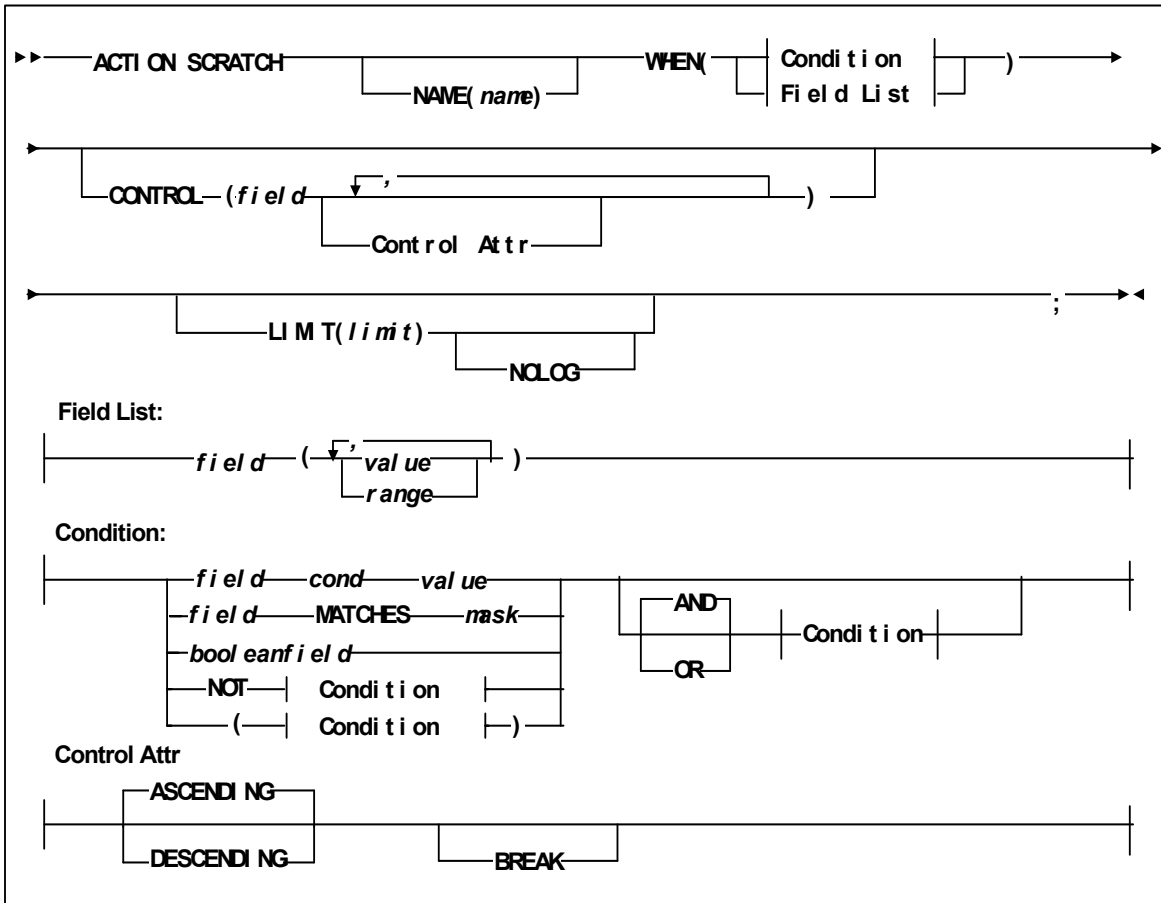
FIGURE 5-11 ACTION SCRATCH Statement Syntax
