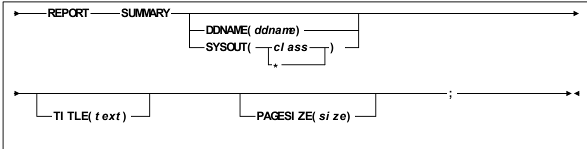
FIGURE 6-21 REPORT SUMMARY Statement Syntax
