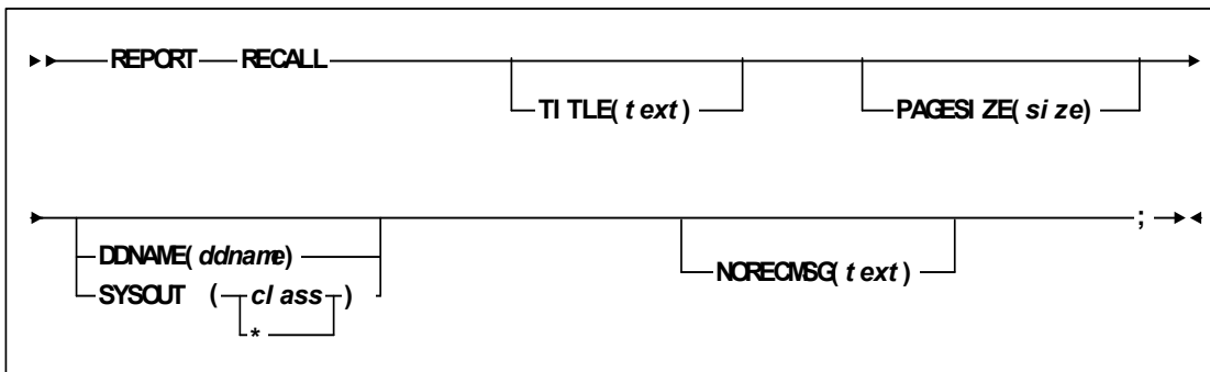
FIGURE 6-17 REPORT RECALL Statement Syntax
