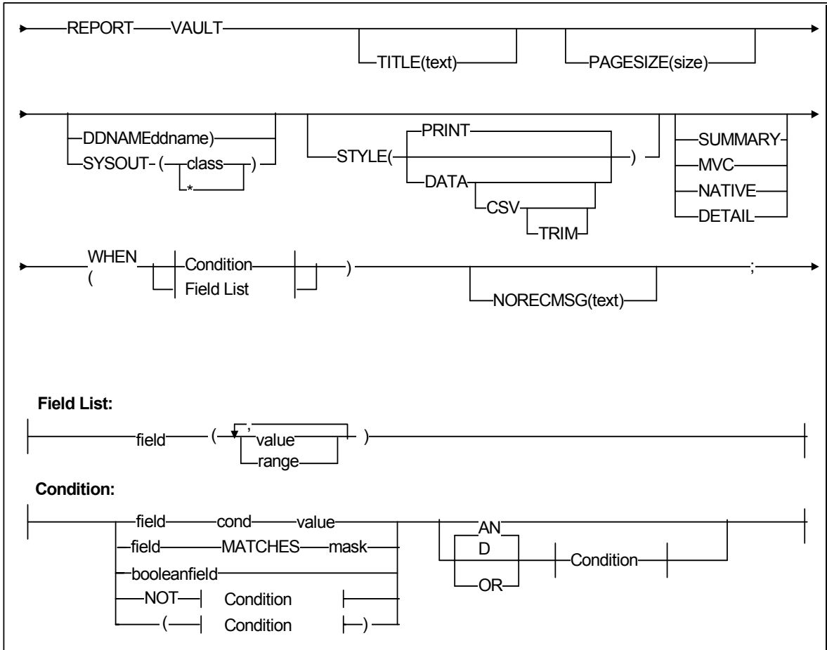
FIGURE 6-27 REPORT VAULT Statement Syntax
