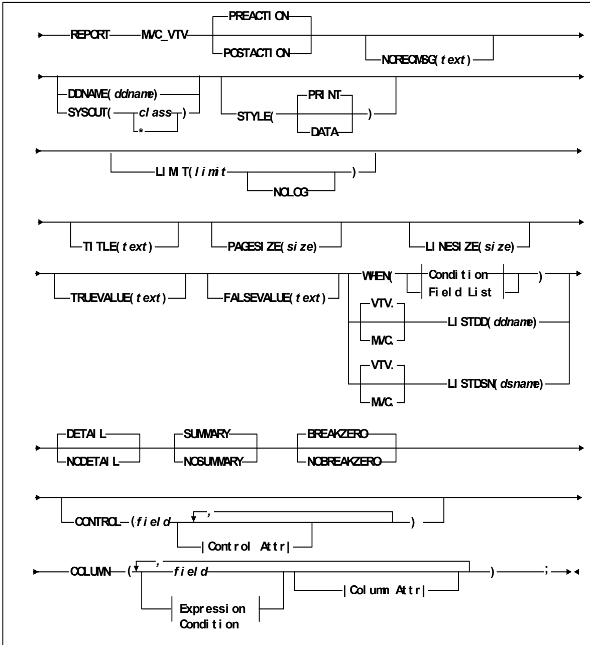
FIGURE 6-37 REPORT MVC_VTV Statement Syntax - Part 1
