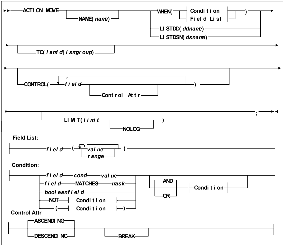
FIGURE 5-6 ACTION MOVE Statement Syntax
