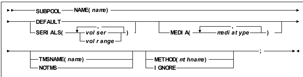
FIGURE 4-14 SUBPOOL Statement Syntax
