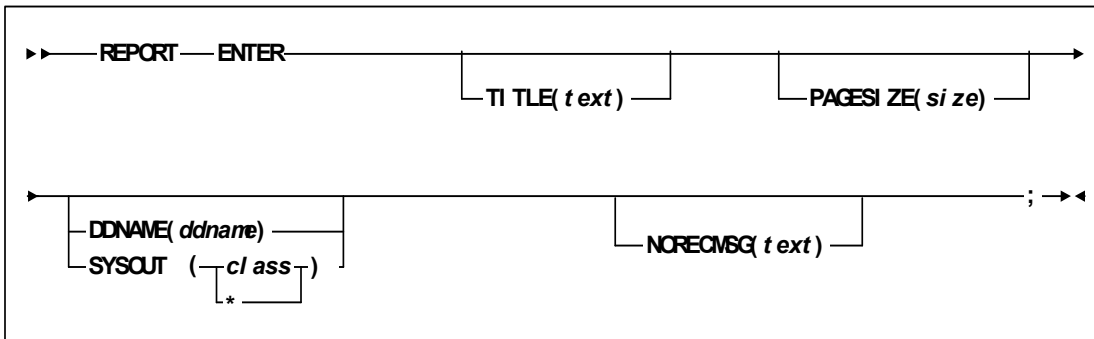
FIGURE 6-7 REPORT ENTER Statement Syntax
