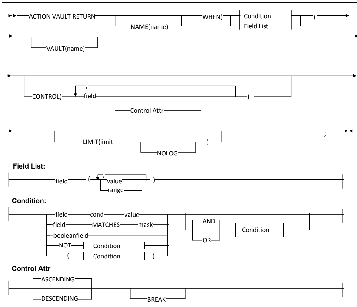
FIGURE 5-15 ACTION VAULT RETURN Statement Syntax
