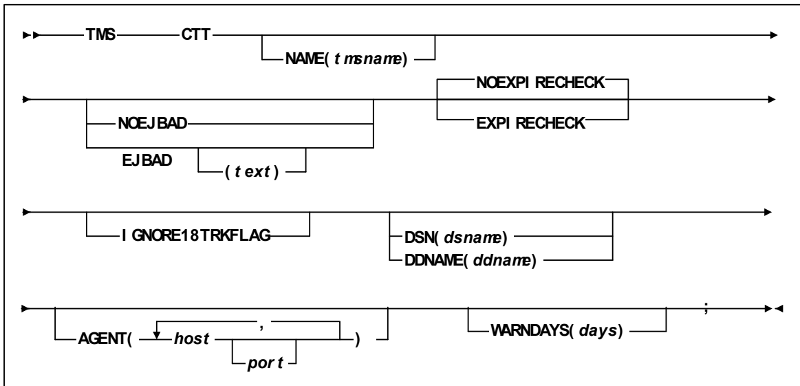
FIGURE 4-22 TMS CTT Statement Syntax
