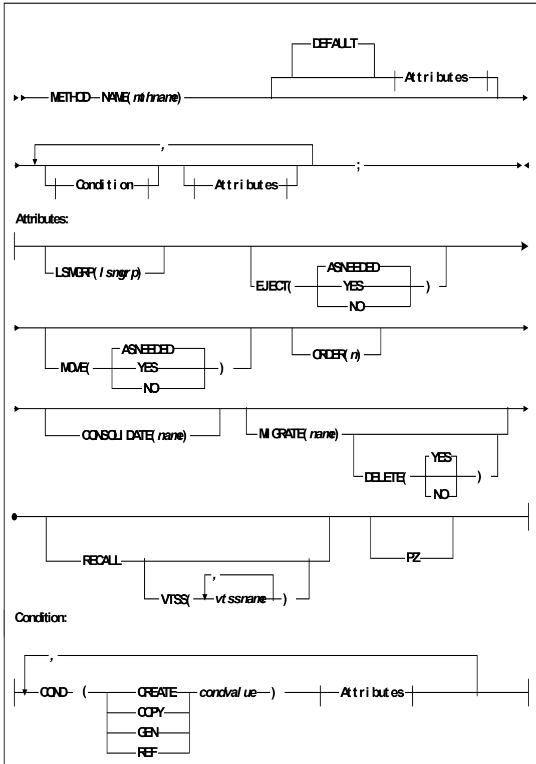
FIGURE 4-5 METHOD Statement Syntax
