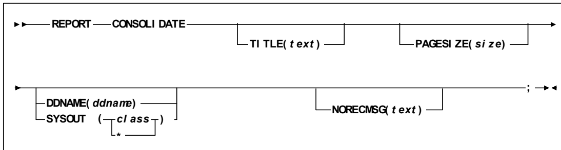
FIGURE 6-3 REPORT CONSOLIDATE Statement Syntax
