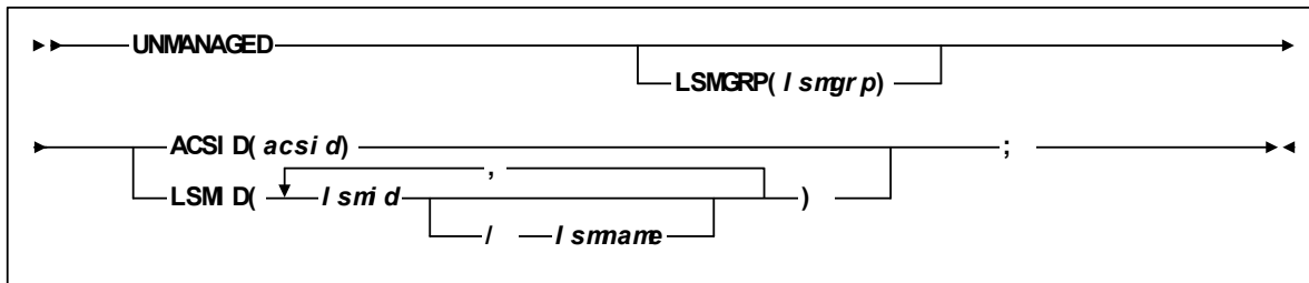
FIGURE 4-27 UNMANAGED Statement Syntax
