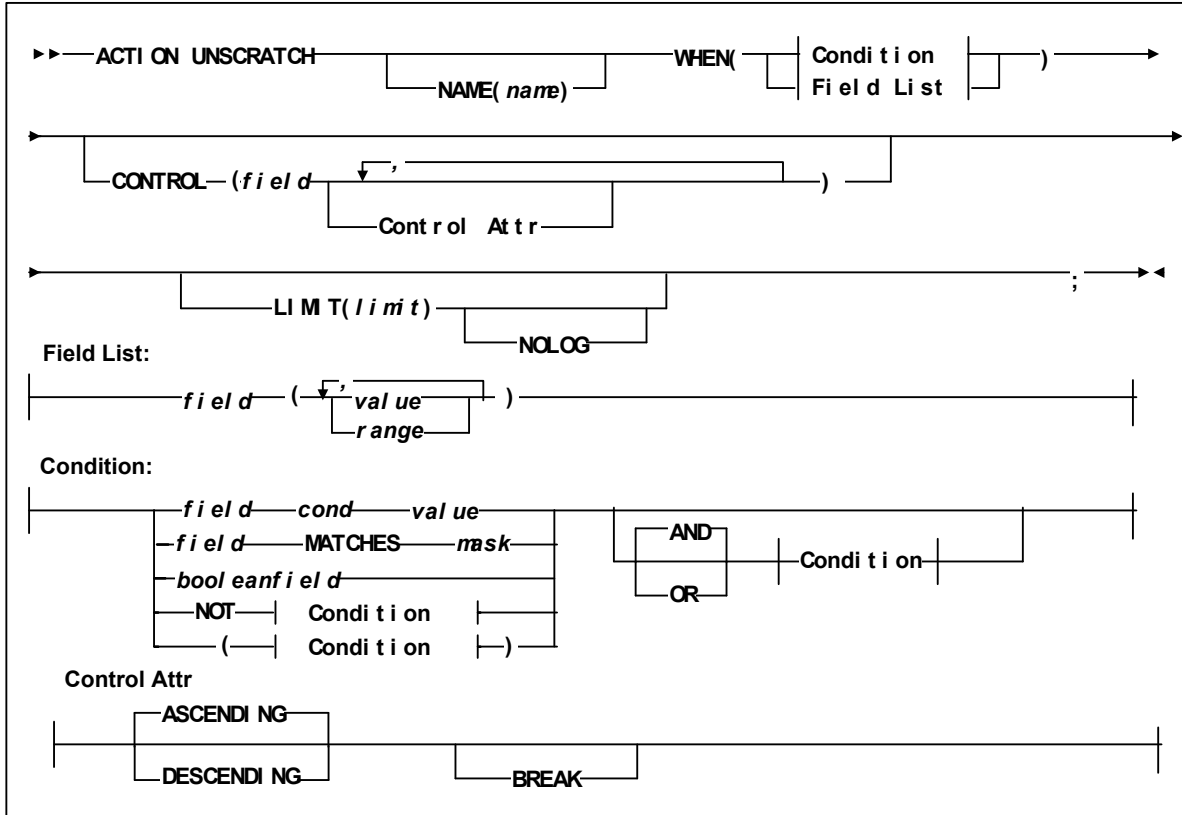
FIGURE 5-12 ACTION UNSCRATCH Statement Syntax
