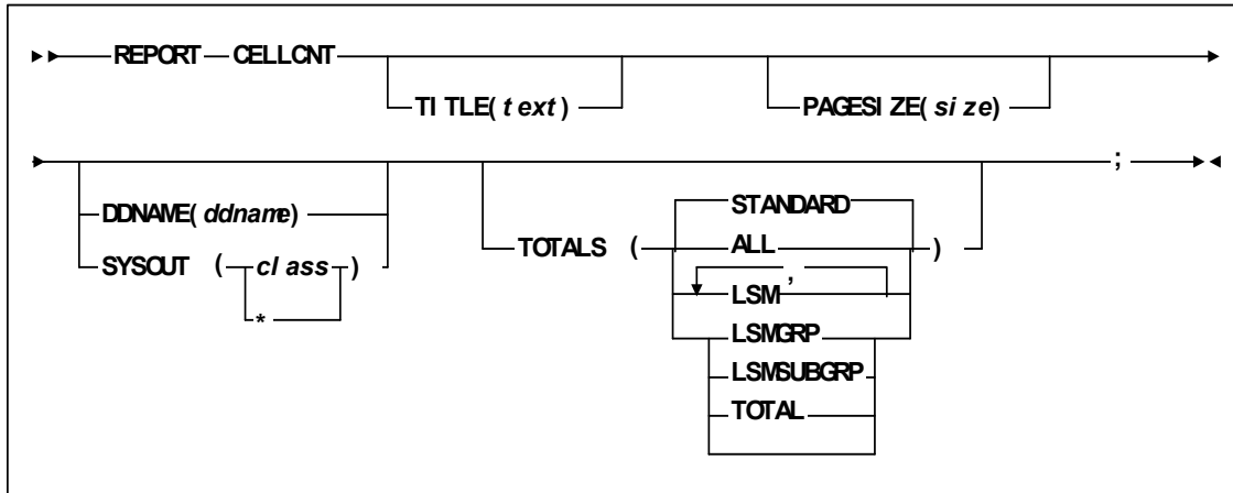
FIGURE 6-1 REPORT CELLCNT Statement Syntax
