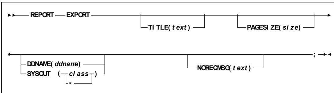
FIGURE 6-9 REPORT EXPORT Statement Syntax
