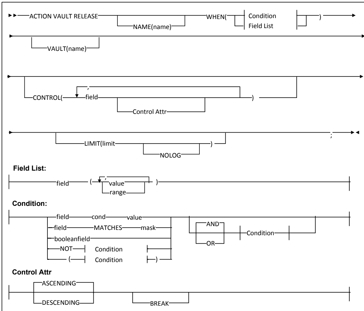
FIGURE 5-14 ACTION VAULT RELEASE Statement Syntax
