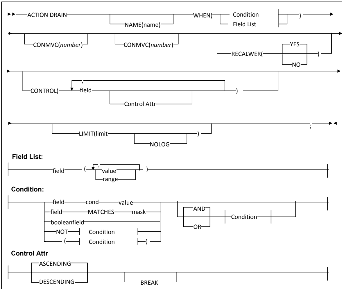
FIGURE 5-2 ACTION DRAIN Statement Syntax
