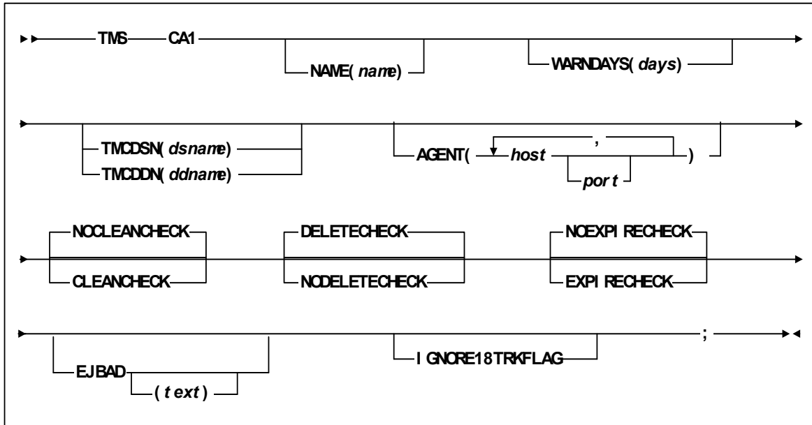
FIGURE 4-20 TMS CA1 Statement Syntax
