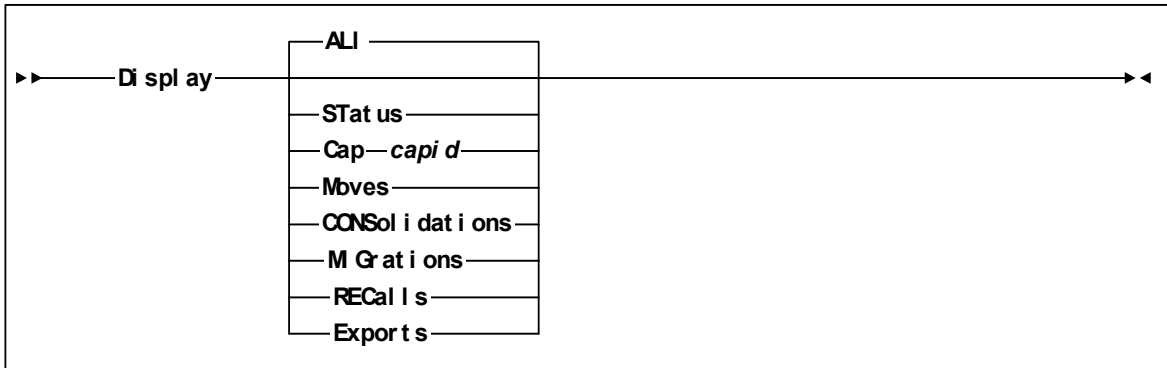
FIGURE 7-1 Display Command Syntax
