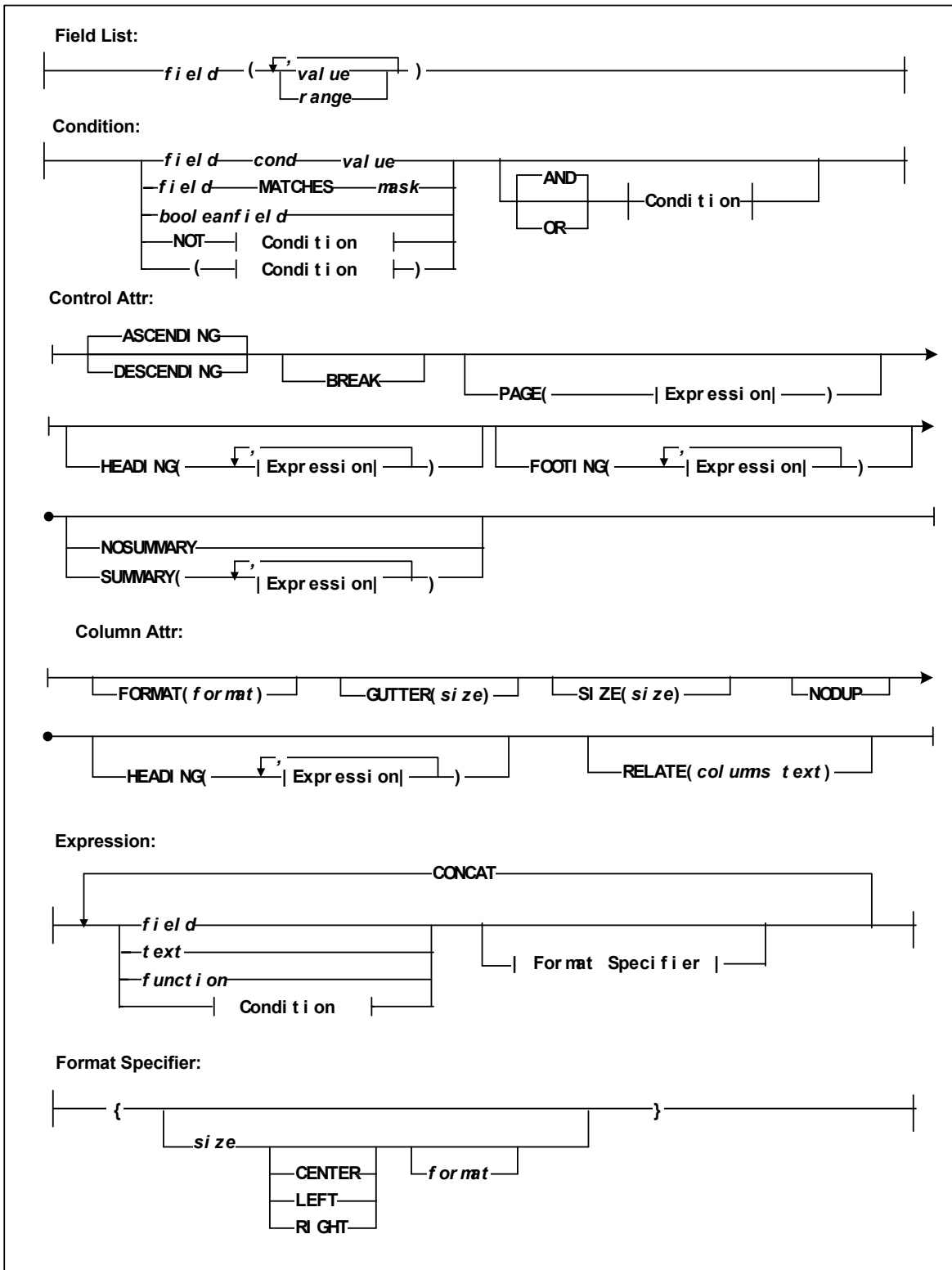
FIGURE 6-36 REPORT LSM Statement Syntax - Part 2
