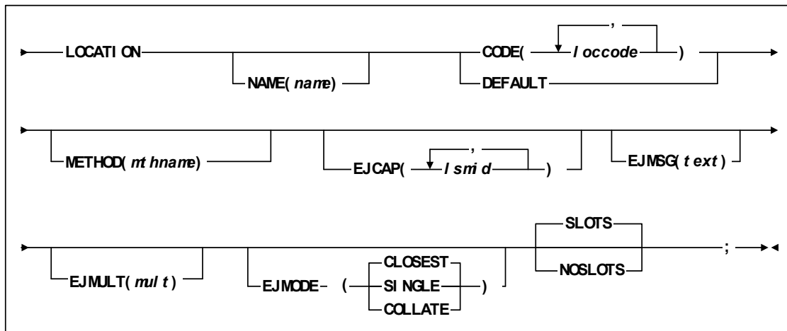
FIGURE 4-2 LOCATION Statement Syntax
