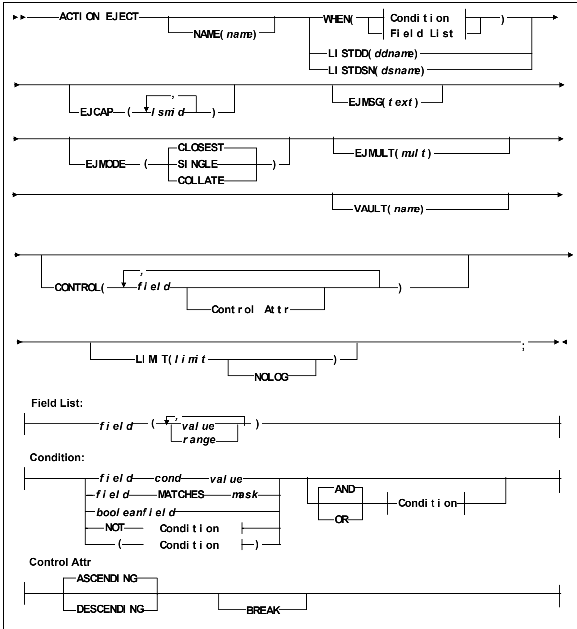
FIGURE 5-3 ACTION EJECT Statement Syntax
