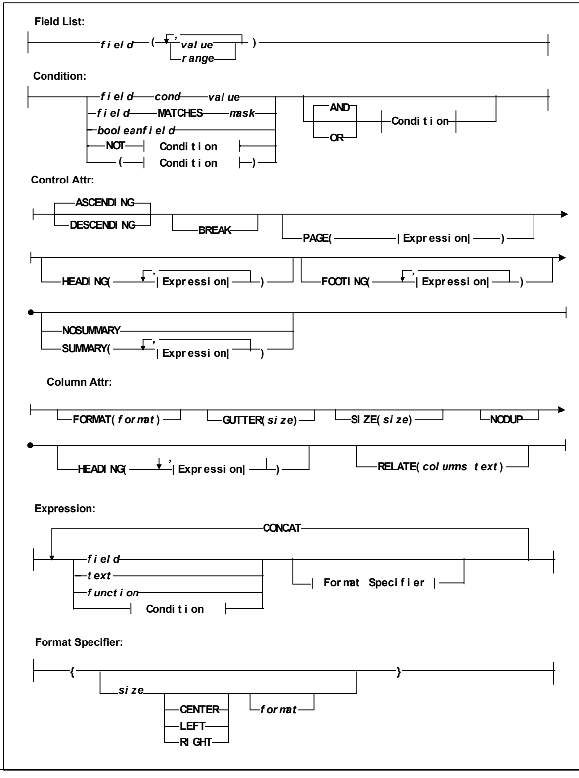
FIGURE 6-38 REPORT MVC_VTV Statement Syntax - Part 2
