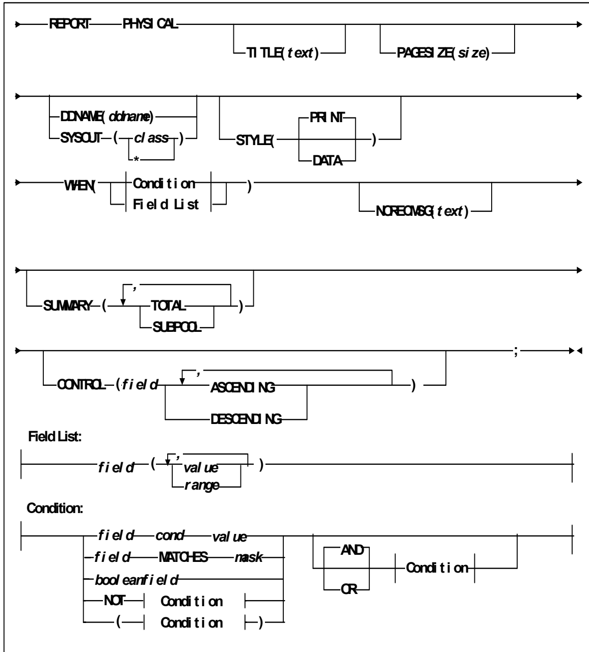
FIGURE 6-26 REPORT PHYSICAL Statement Syntax
