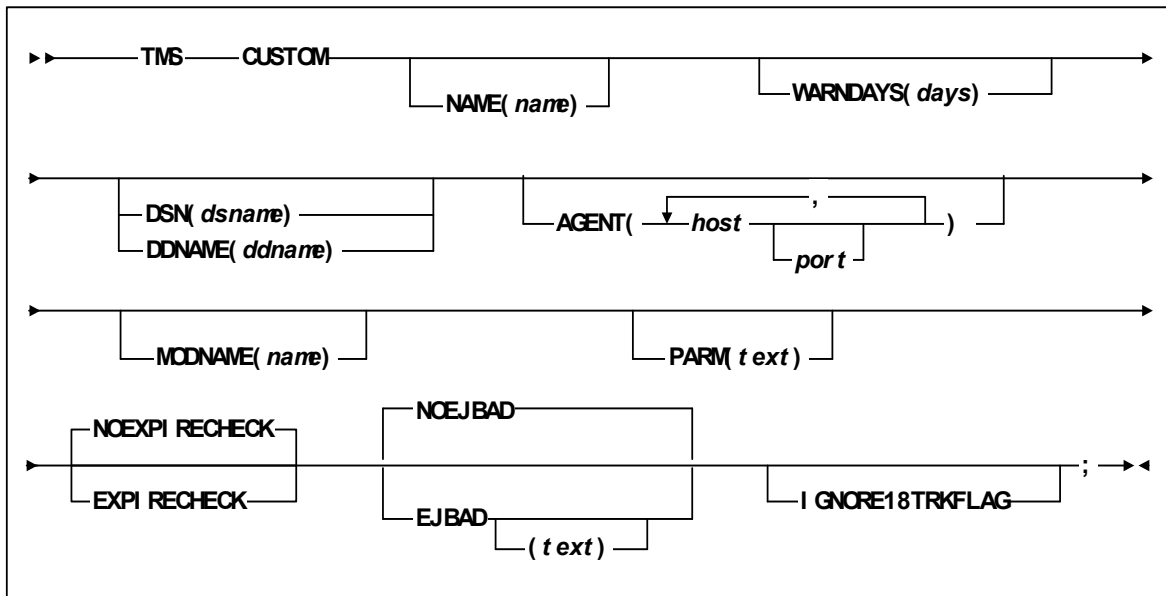
FIGURE 4-23 TMS CUSTOM Statement Syntax
