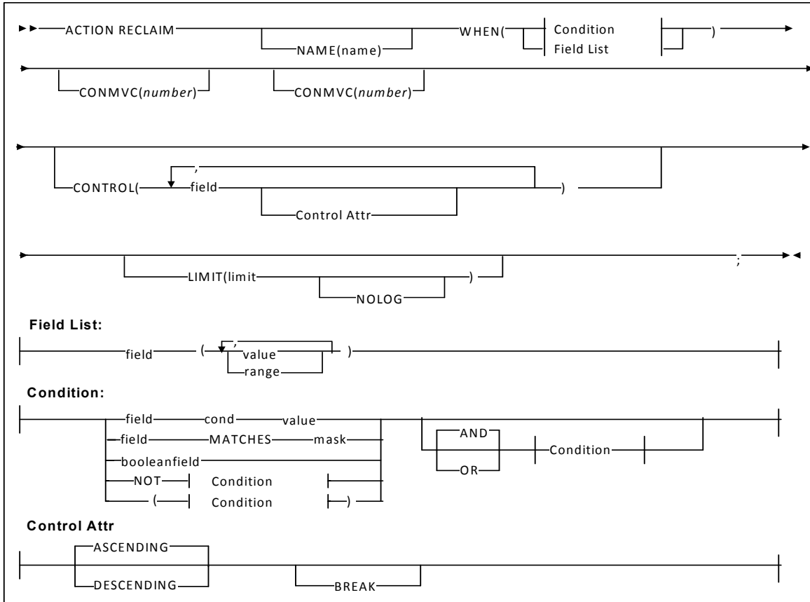
FIGURE 5-10 ACTION RECLAIM Statement Syntax
