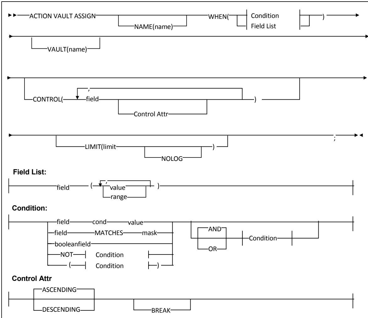
FIGURE 5-13 ACTION VAULT ASSIGN Statement Syntax
