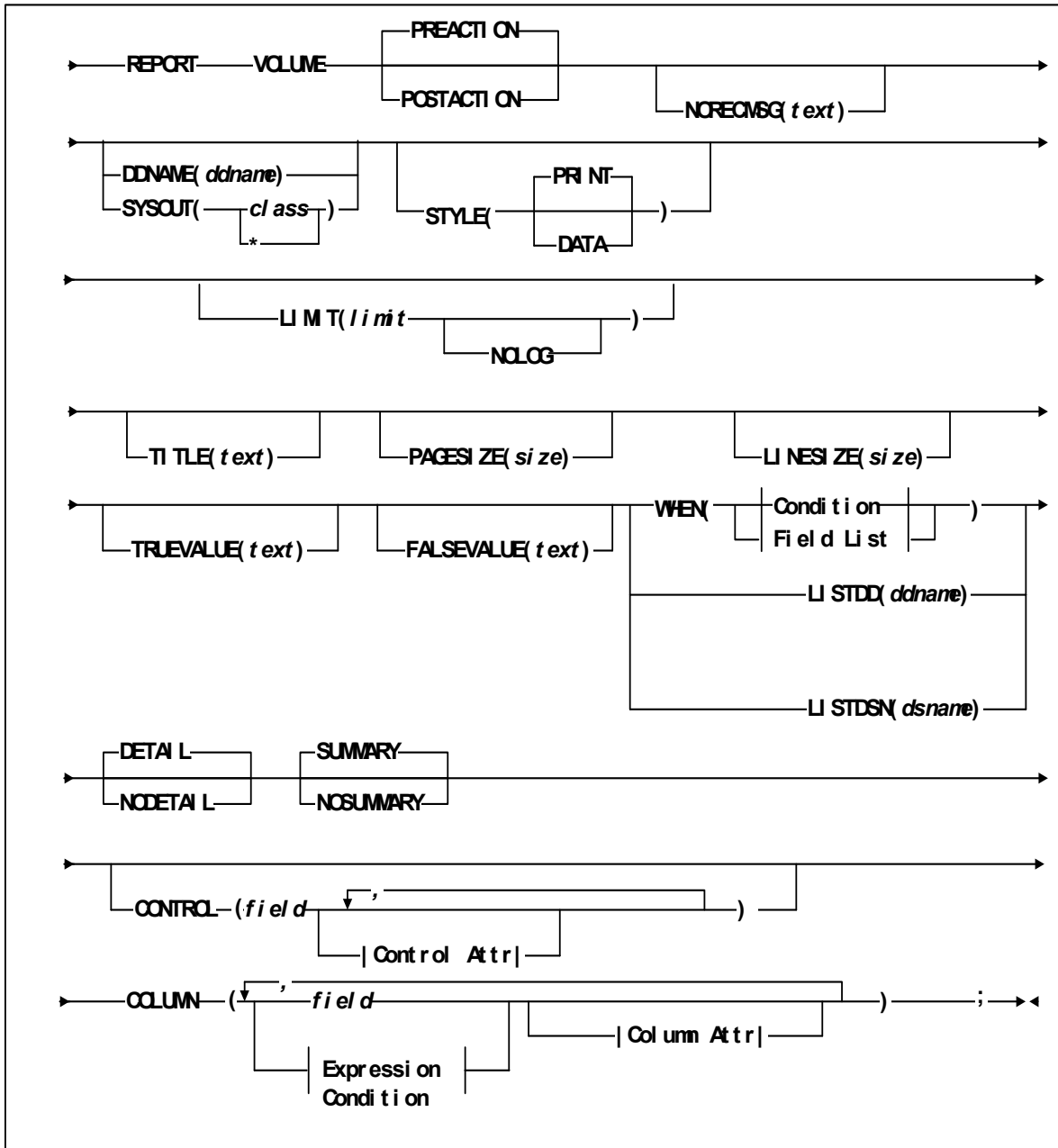
FIGURE 6-39 REPORT VOLUME Statement Syntax - Part 1
