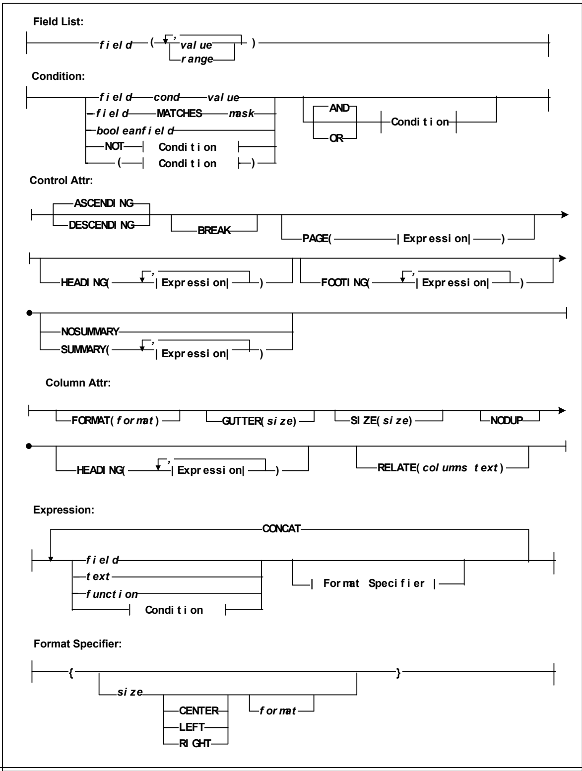
FIGURE 6-40 REPORT VOLUME Statement Syntax - Part 2
