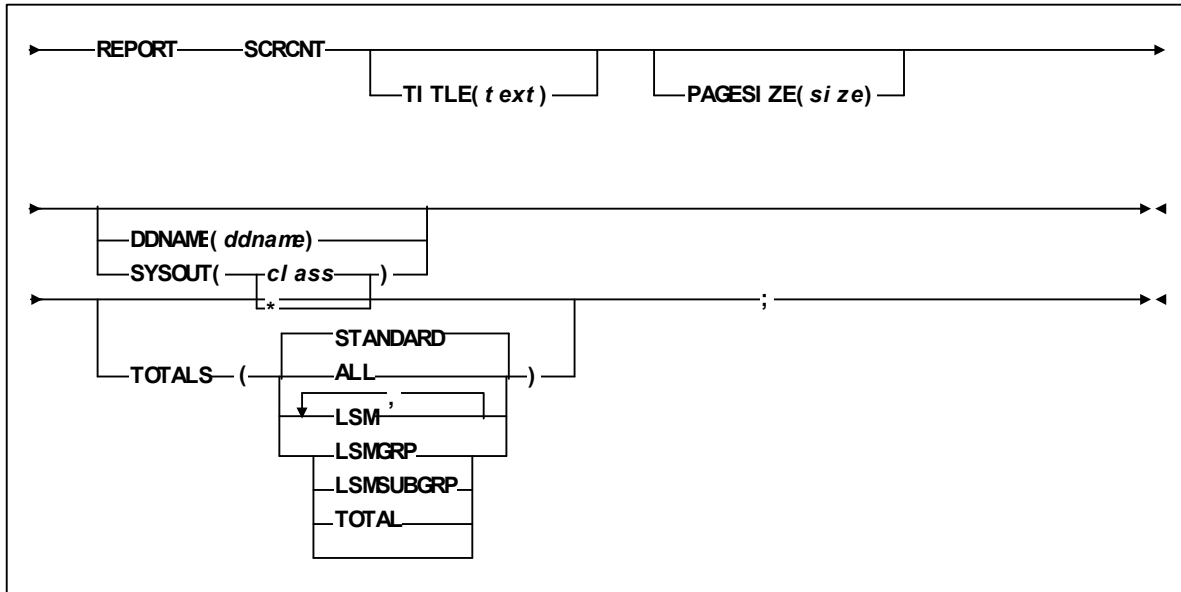
FIGURE 6-19 REPORT SCRCNT Statement Syntax
