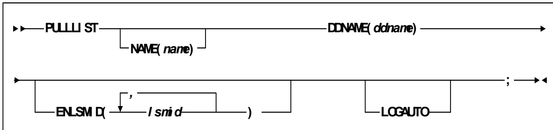
FIGURE 4-11 PULLLIST Statement Syntax
