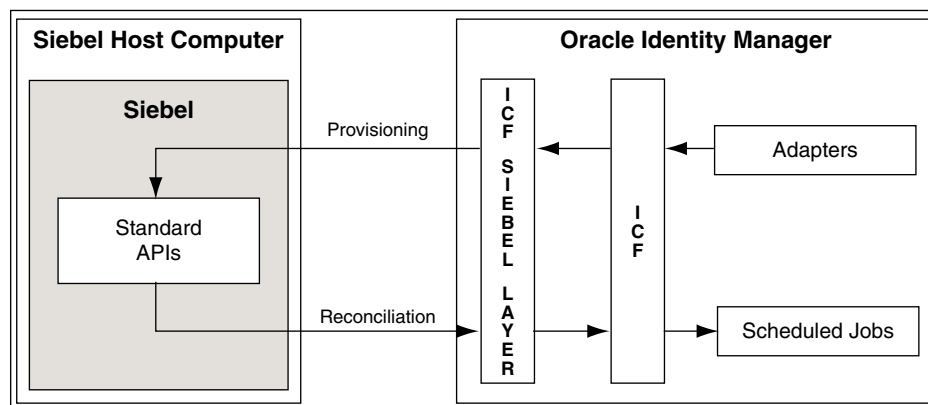
Figure 1-1 Connector Architecture
