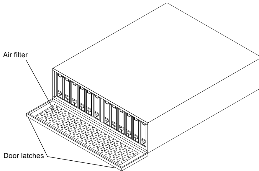
FIGURE 1 Removing and Replacing the Air Filter
