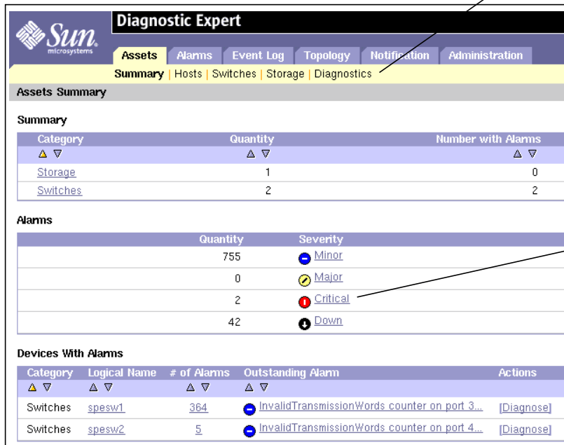
FIGURE 3-4 Assets Window
