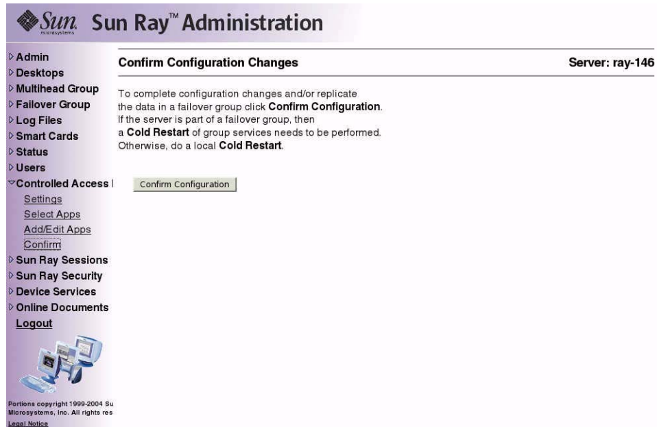
FIGURE 3-37 Confirmation Window
