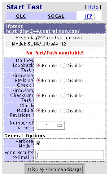
FIGURE 5-9 IFP Test Options Dialog Box
