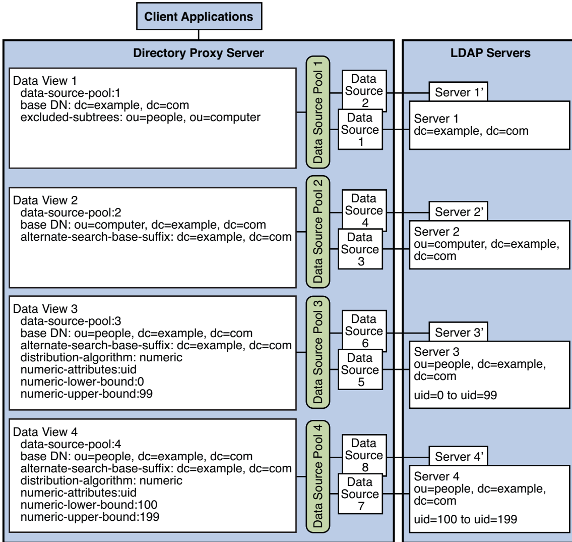
FIGURE 22-8 Data View With Hierarchy and a Distribution Algorithm
