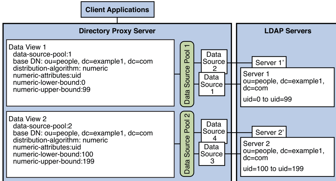
FIGURE 22–6 Example Deployment That Routes Requests When Different Parts of a Subtree Are Stored in Different Data Sources
