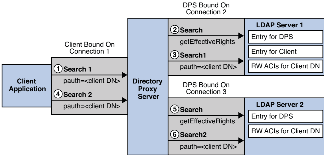
FIGURE 24-4 Information Flow When Proxy Authorization Control Is Contained in the Client Request
