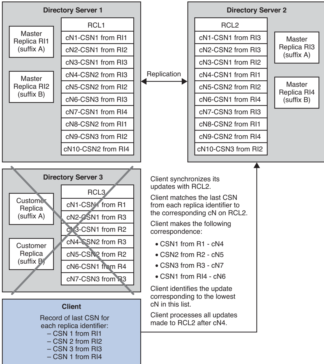
FIGURE 4-9 Failover of the Retro Change Log
