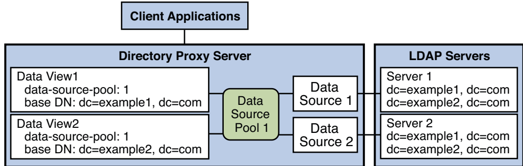
FIGURE 22-4 Example Deployment That Routes Requests When a List of Subtrees Is Stored on Multiple, Data-Equivalent Data Sources
