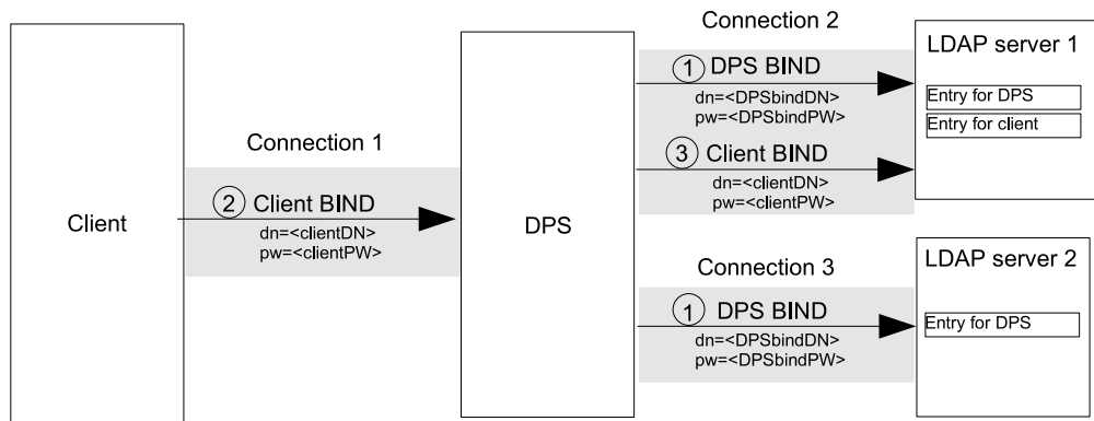
FIGURE 24–2 Connections for Proxy Authorization
