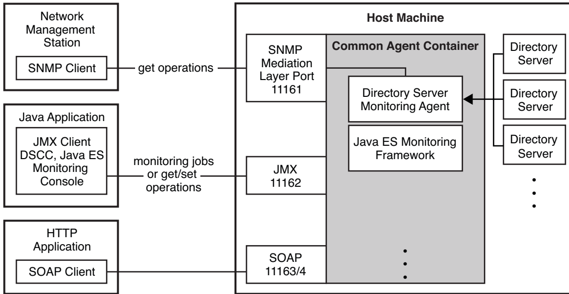
FIGURE 3–1 Overall Monitoring Information Flow
