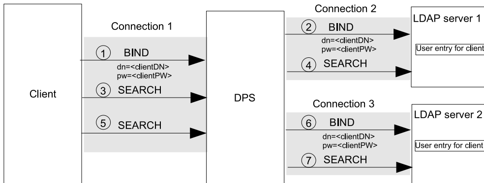
FIGURE 24-1 Authentication in BIND Replay
