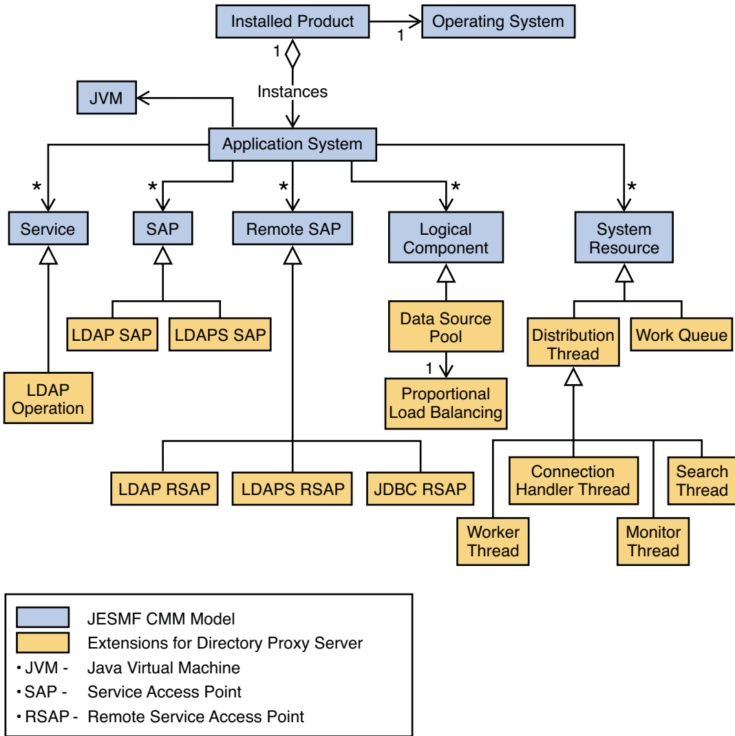
FIGURE 18-1 Monitoring Framework for Directory Proxy Server
