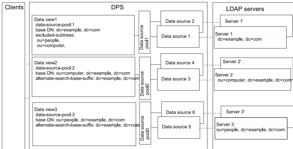
FIGURE 22-7 Example Deployment to Route Requests When Superior and Subordinate Subtrees Are Stored in Different Data Sources
