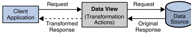
FIGURE 23-4 Read Transformation
