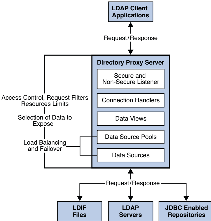
FIGURE 16-1 Simplified Architecture of Directory Proxy Server
