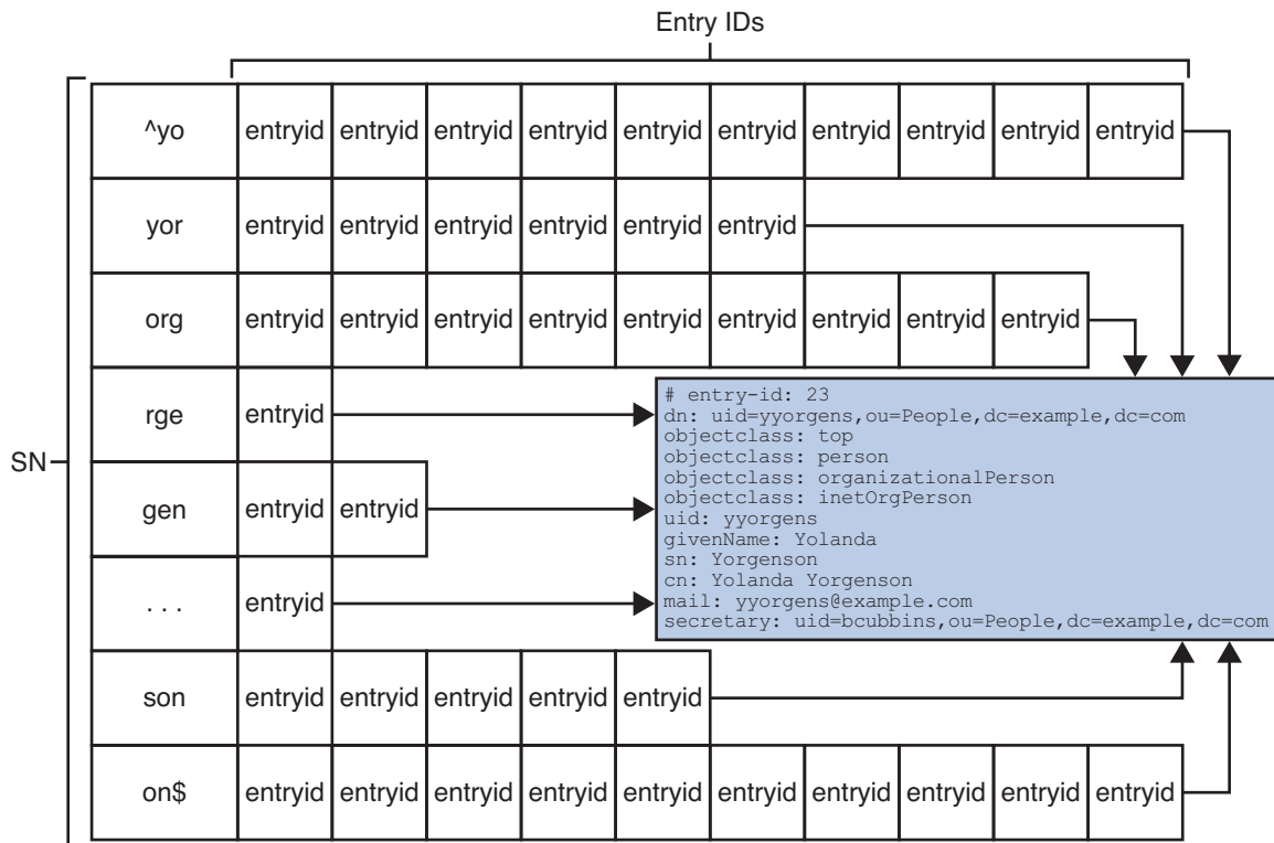
FIGURE 6-3 Substring Index for the SN Attribute
