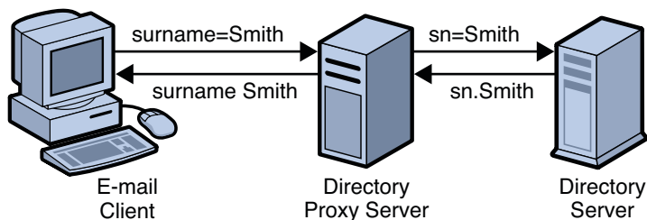
FIGURE 22-1 Attribute Renaming
