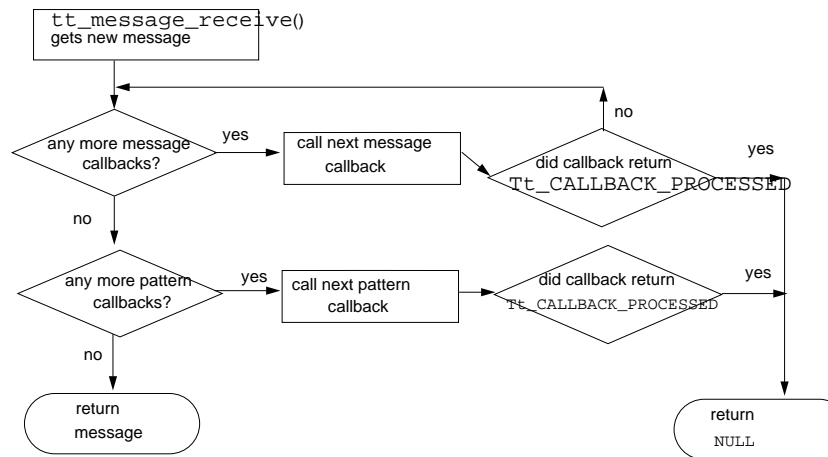
Figure 11-1 How Callbacks Are Invoked
