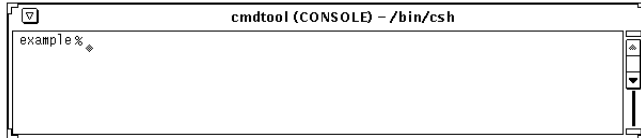
Figure 18-5 Console Window
