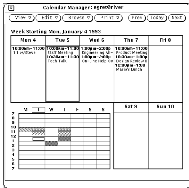
Figure 5-5 Week View
