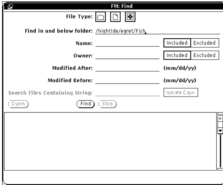
Figure 2-25 Find Window
