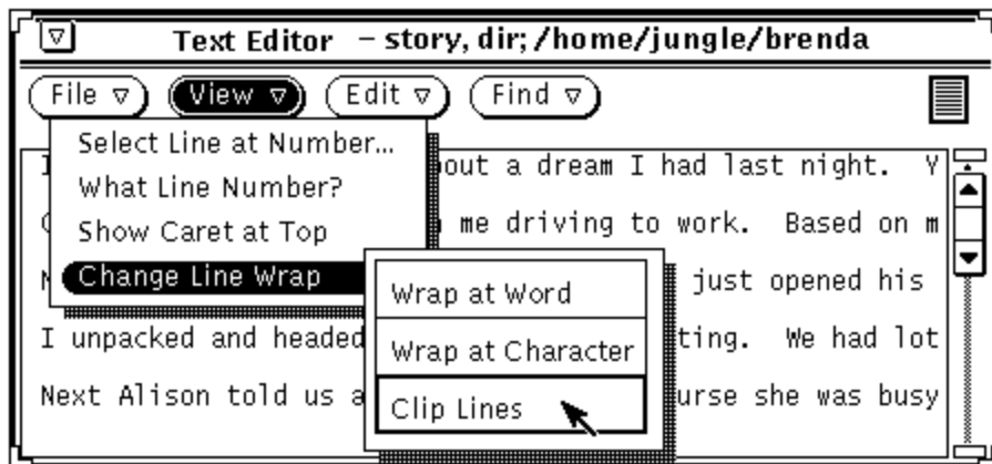
Figure 3-5 Clipped Lines
