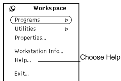
Figure 1-36 Workspace Menu
