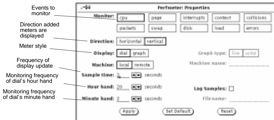
Figure 9-6 The Performance Meter Properties Window
