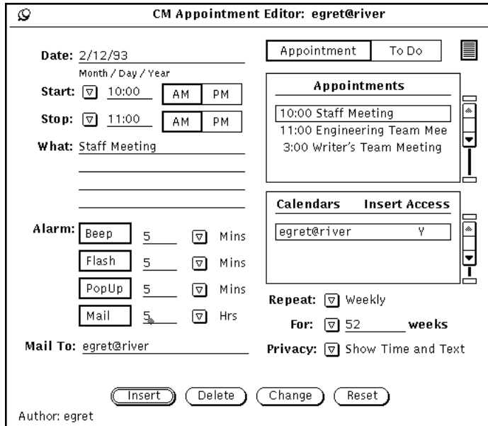
Figure 5-9 Calendar Manager Appointment Window
