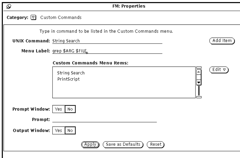
Figure 2-45 Custom Command Pop-up Window
