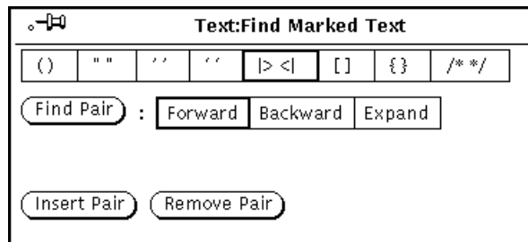
Figure 3-7 Text: Find Marked Text Pop-up Window
