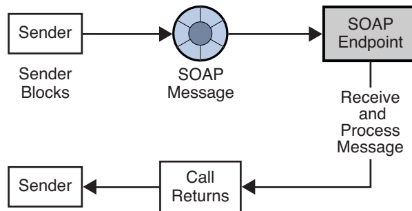
FIGURE 5–6 Request-Reply Messaging
