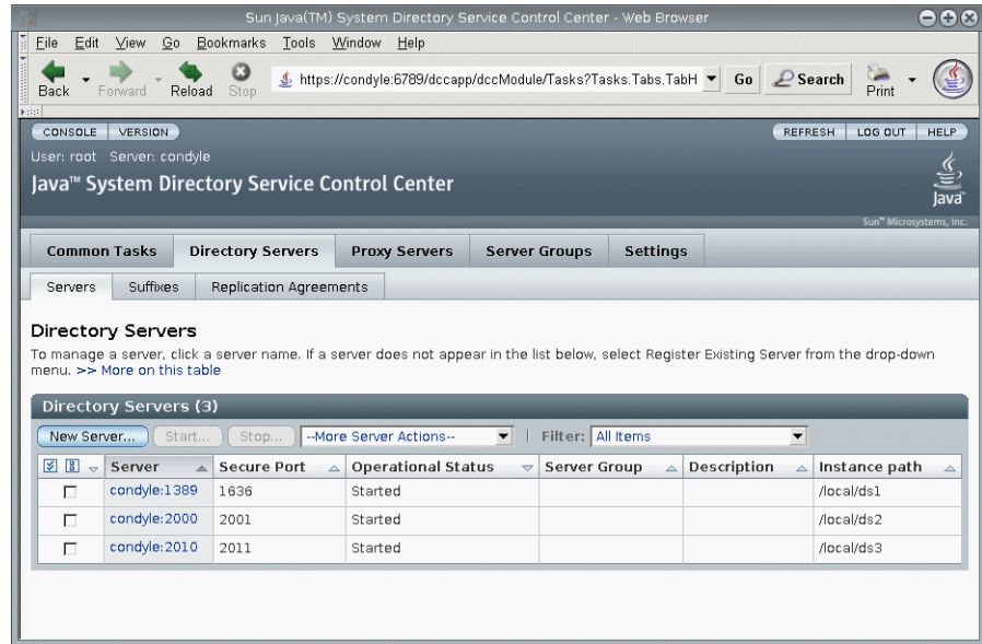
FIGURE 2-3 List of Directory Servers On the Servers Sub Tab
