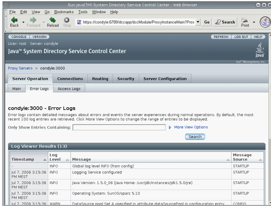
FIGURE 28-1 Error Log Window for Directory Proxy Server
