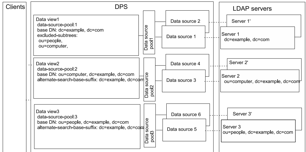
FIGURE 19-3 Sample Deployment to Routes Requests When Superior and Subordinate Subtrees Are Stored in Different Data Sources
