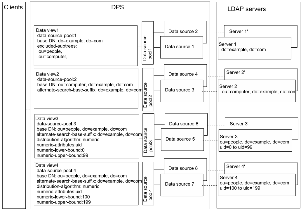
FIGURE 22-2 Sample Data View With Hierarchy and a Distribution Algorithm
