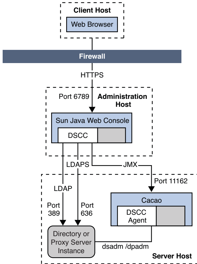
FIGURE 1-2 Administration Host and Server Host on Different Systems After Installation of Native Packages Distribution
