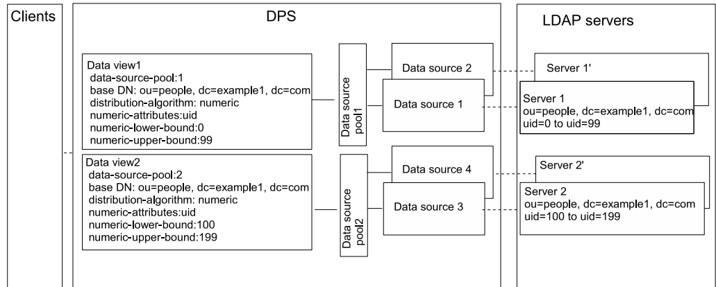
FIGURE 22-1 Sample Deployment That Provides a Single Point of Access When Different Parts of a Subtree Are Stored in Different Data Sources
