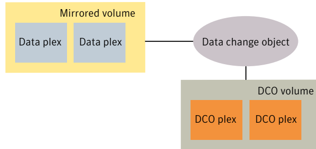
Figure 1-33 Mirrored volume with persistent FastResync enabled
