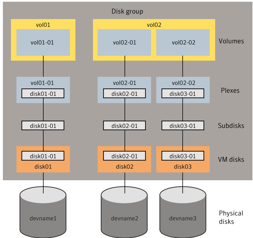
Figure 1-6 Connection between objects in VxVM
