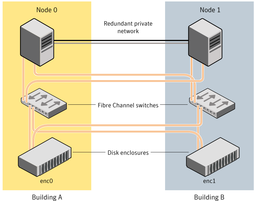
Figure 5-1 Typical arrangement of a 2-node campus cluster
