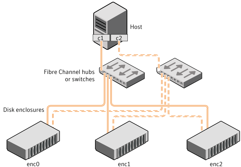
Figure 1-5 Example HA configuration using multiple hubs or switches to provide redundant loop access
