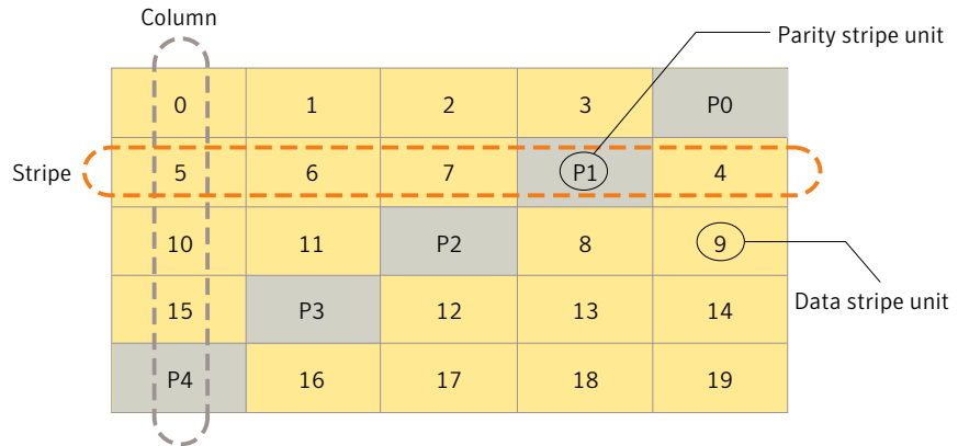
Figure 1-24 Left-symmetric layout
