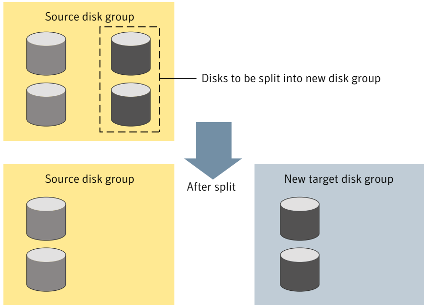
Figure 5-5 Disk group split operation
