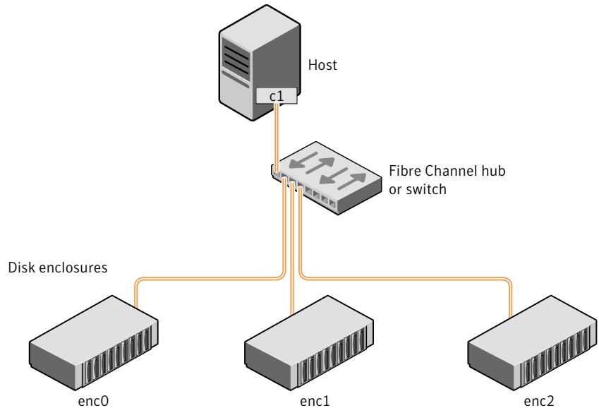
Figure 1-4 Example configuration for disk enclosures connected via a fibre channel hub or switch
