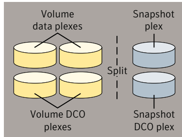
Figure 5-7 Examples of disk groups that can and cannot be split
