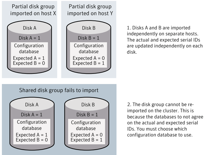
Figure 5-3 Example of a true serial split brain condition that cannot be resolved automatically
