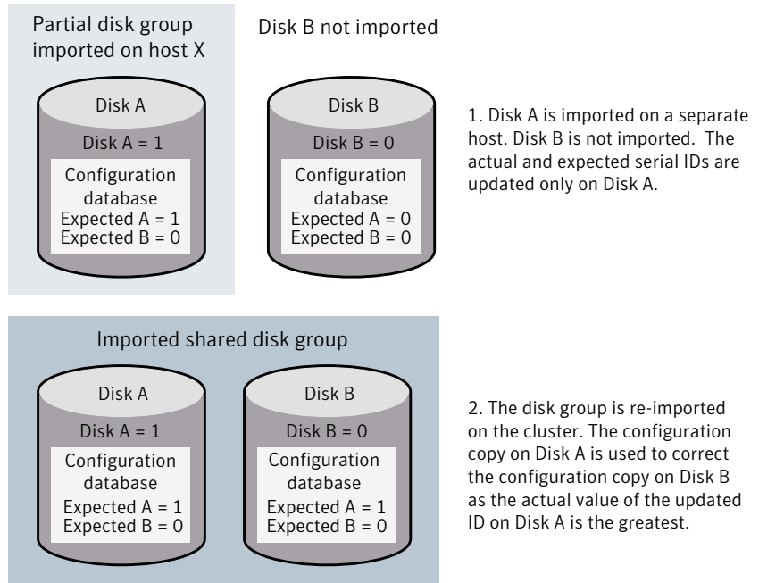
Figure 5-2 Example of a serial split brain condition that can be resolved automatically
