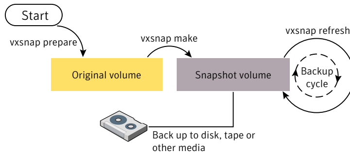
Figure 9-3 Space-optimized instant snapshot creation and usage in a backup cycle
