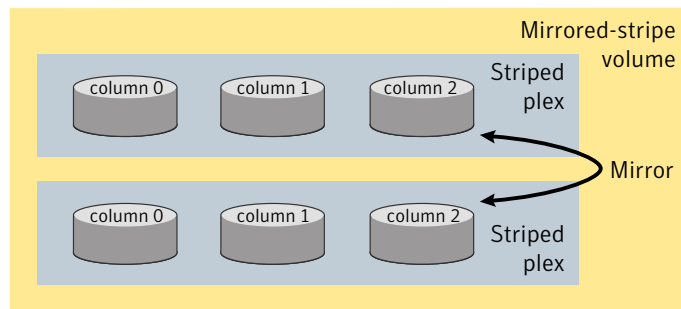
Figure 1-18 Mirrored-stripe volume laid out on six disks
