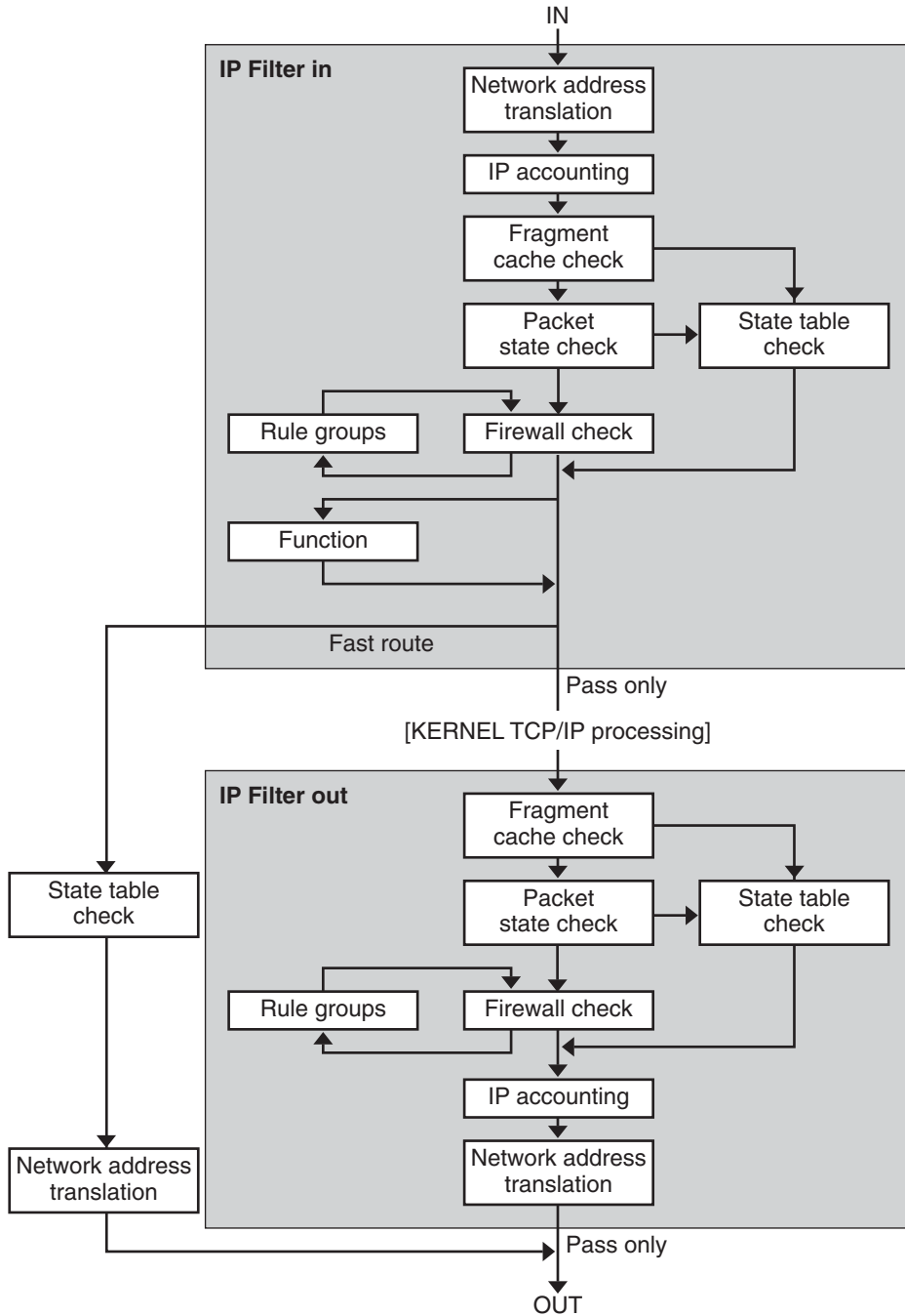
FIGURE 24-1 Packet Processing Sequence
