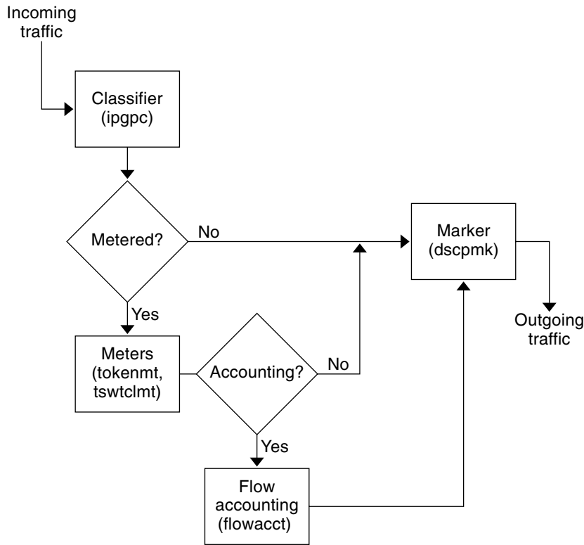
FIGURE 26-1 Traffic Flow Through the IPQoS Implementation of the Diffserv Model
