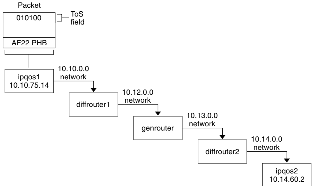
FIGURE 26-2 Packet Forwarding Across Diffserv-Aware Network Hops
