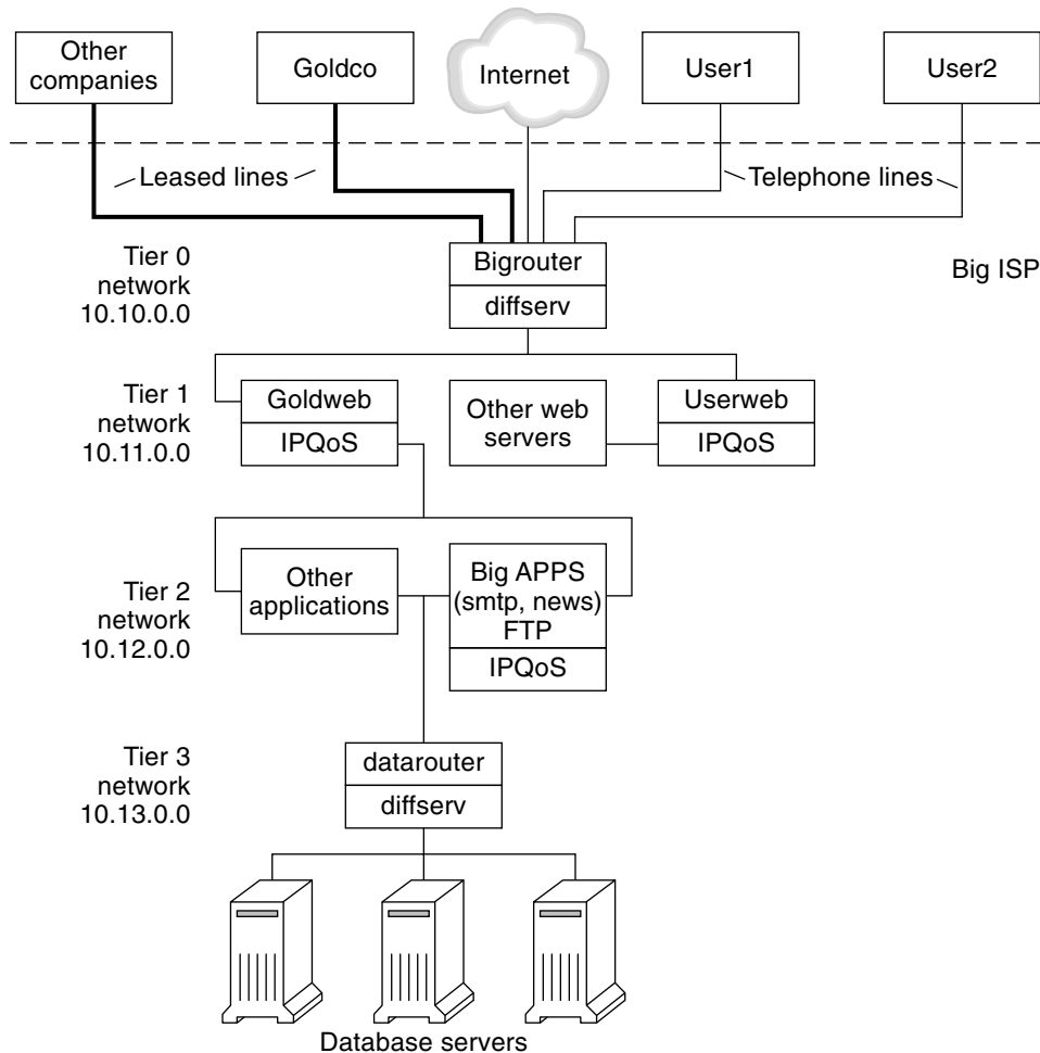
FIGURE 27-4 IPQoS Example Topology
