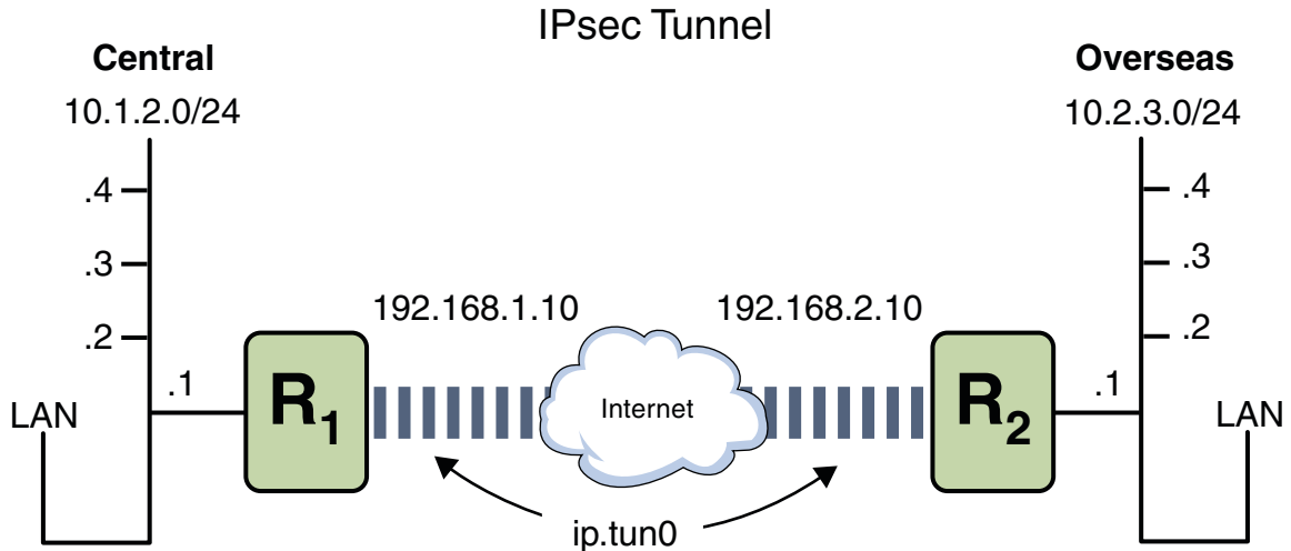
FIGURE 19-1 IPsec Tunnel Diagram
