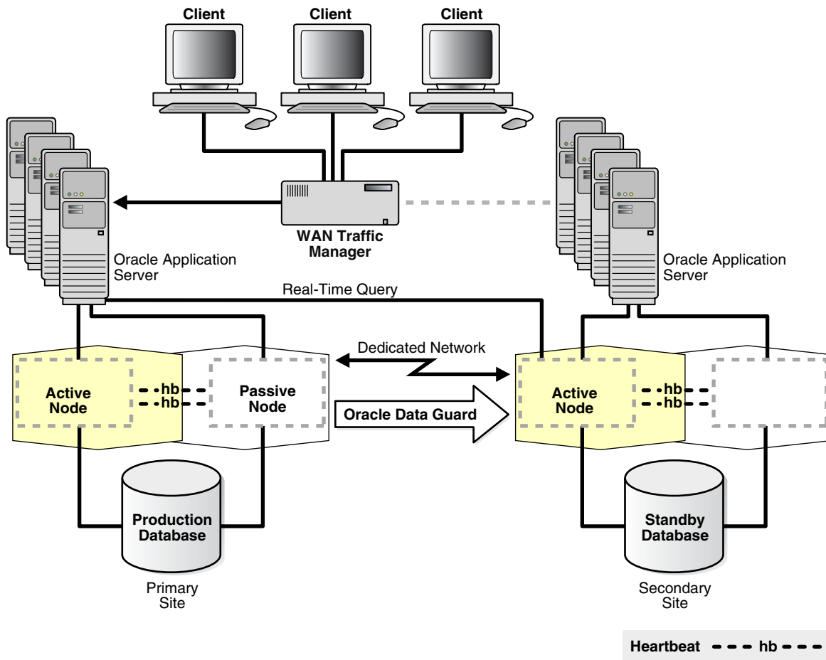
Figure 7–8 Oracle Clusterware (Cold Cluster Failover) and Oracle Data Guard
