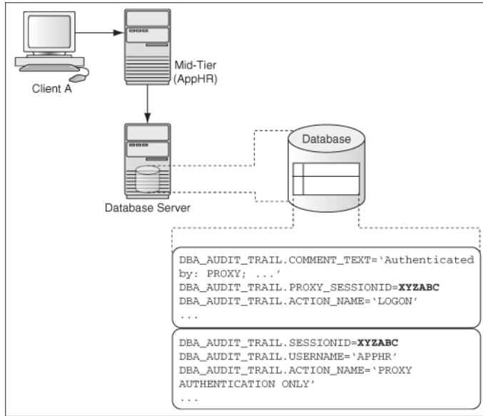
Figure 9–1 Auditing Proxy Users
