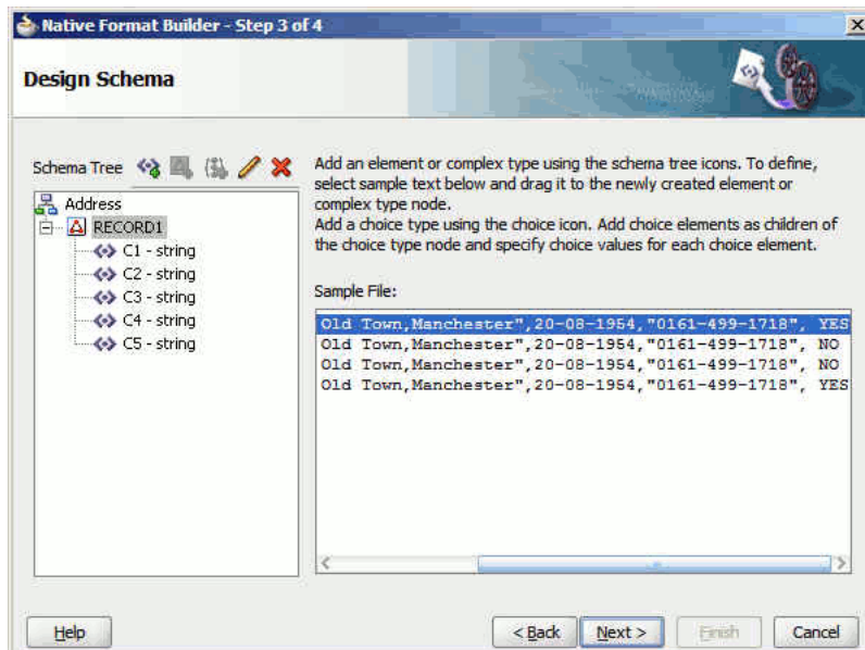
Figure 6-52 Native Format Builder Design Schema Page
