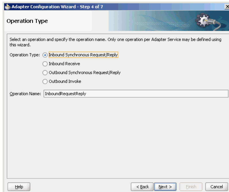
Figure 5–46 The Adapter Configuration Wizard Operation Page
