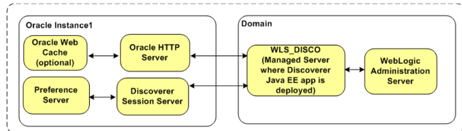
Figure 14-5 Discoverer Topology for a Single Instance
