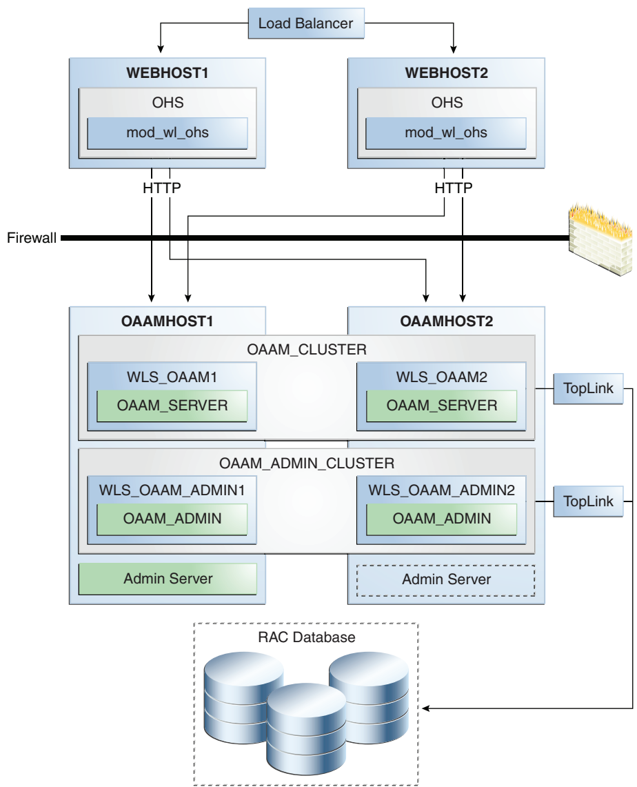
Figure 8–19 Oracle Adaptive Access Manager High Availability Architecture
