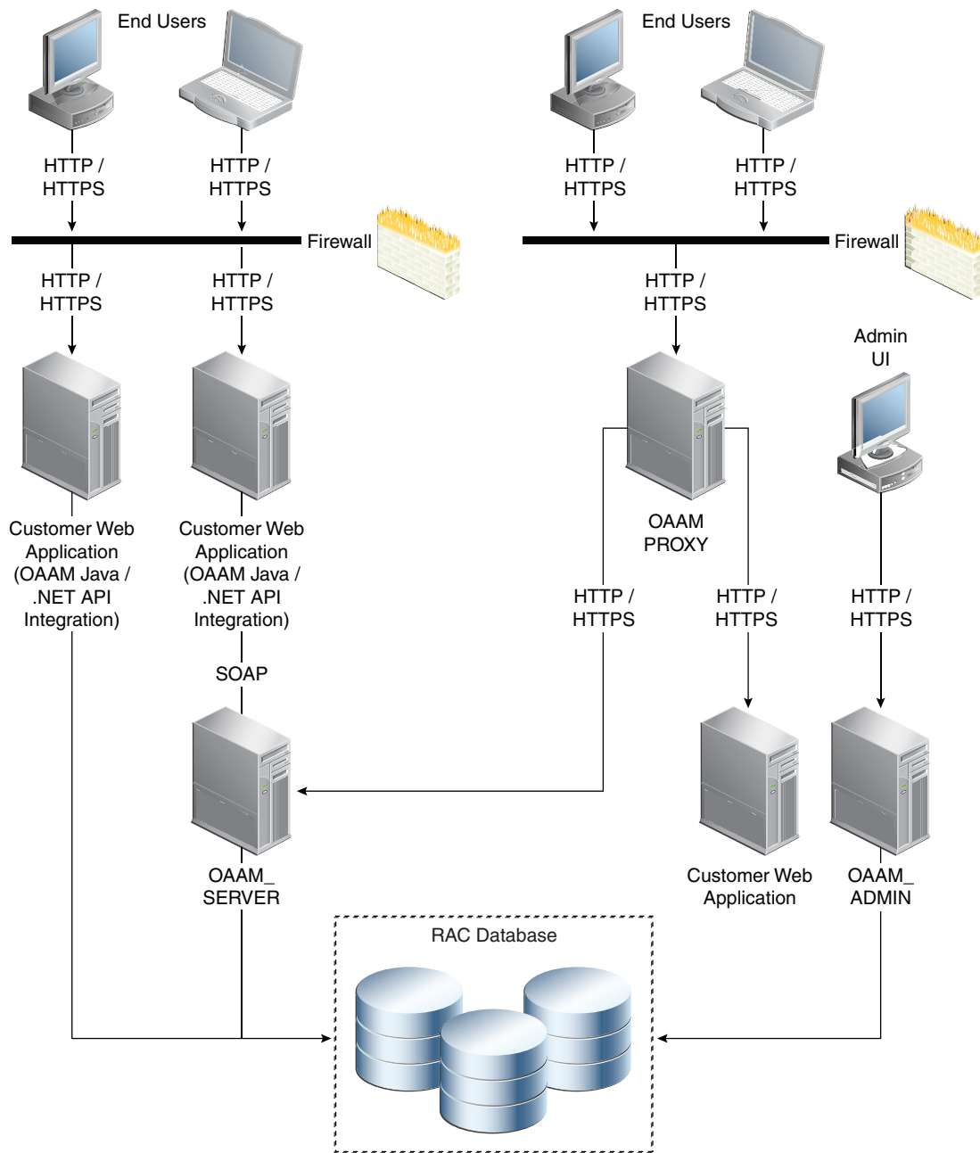
Figure 8–18 Oracle Adaptive Access Manager Single Instance Architecture
