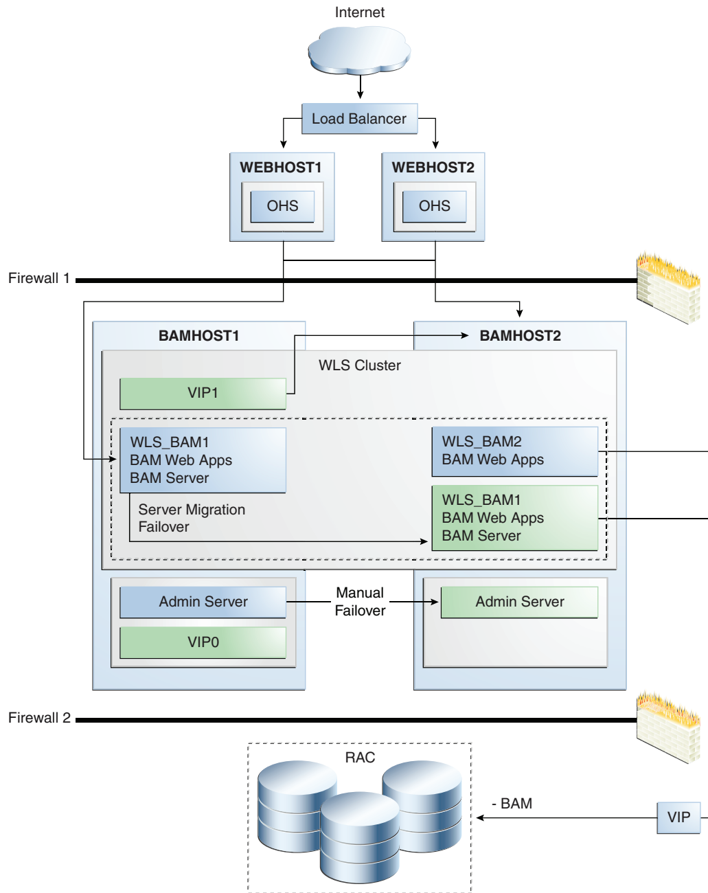
Figure 5–53 illustrates a two-node cluster running Oracle BAM Web Applications. One of them is also running Oracle BAM Server. The Oracle WebLogic Servers are fronted by Oracle HTTP Servers, which load balance incoming requests to BAM Web Applications. A load balancer front ends the system and distributes requests from clients to the two HTTP Servers. An Oracle RAC database stores metadata and BAM schemas.
