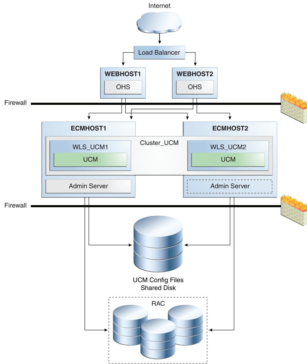
Figure 11–4 Oracle Universal Content Management Two-Node Cluster
