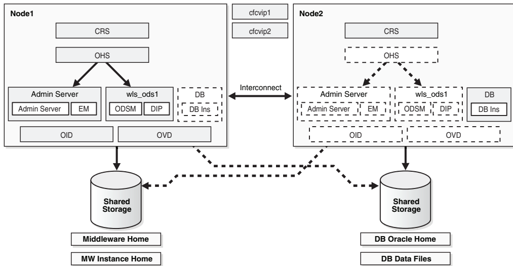
Figure 12-5 Cold Failover Cluster Example Topology 3
