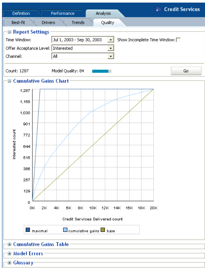
Figure 2–35 Choice Group Cumulative Gains Chart
