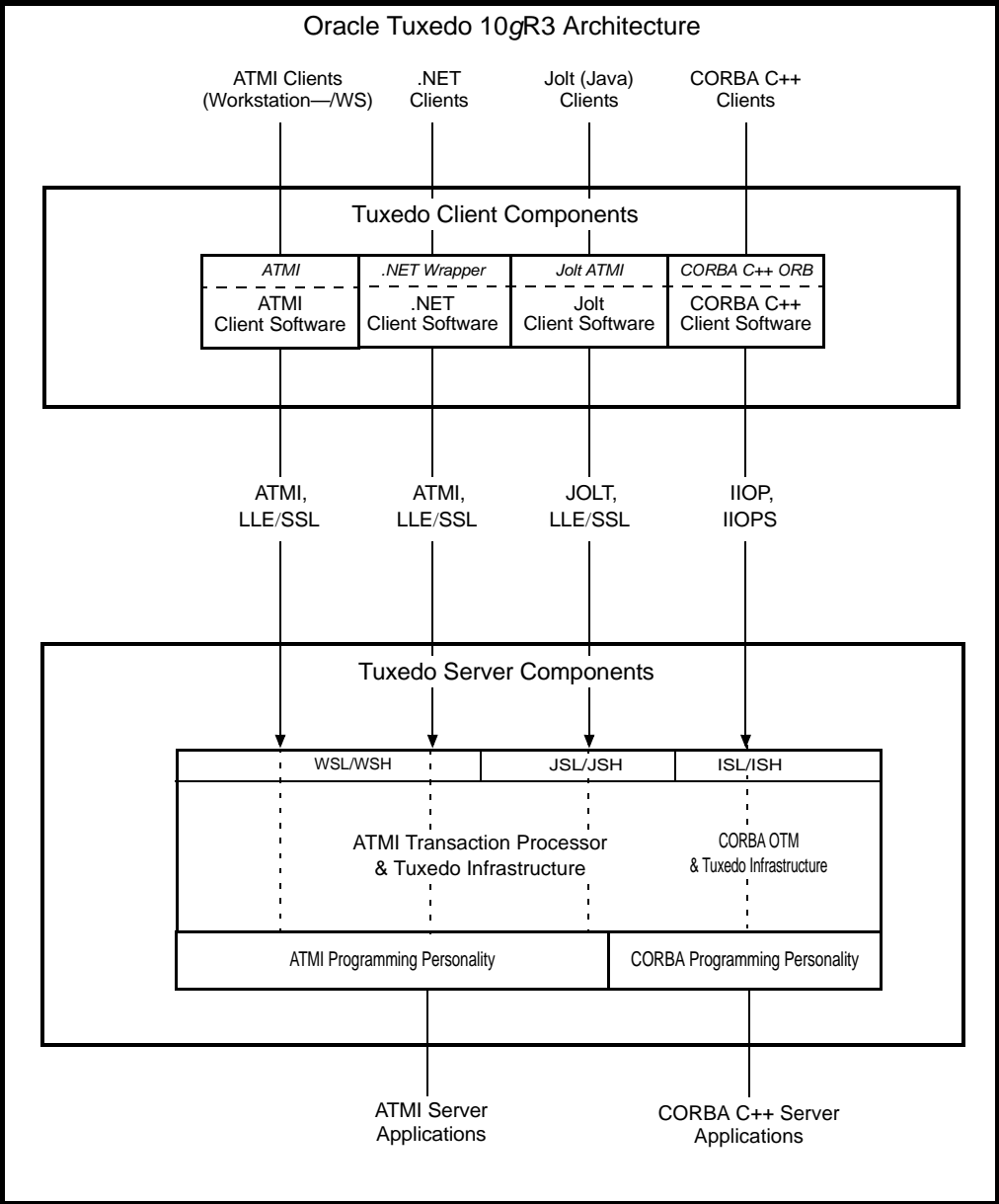
Figure 1-1 Oracle Tuxedo Client and Server Components
