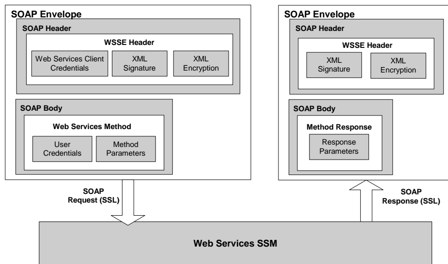
Figure 2-8 SOAP Message Format
