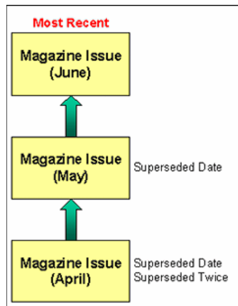
Figure 3-8 Supersedes relationship
