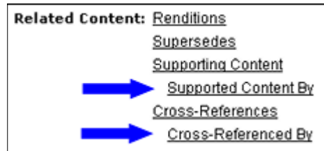
Figure 4–7 Destination links
