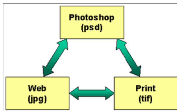
Figure 3–7 Renditions relationship
