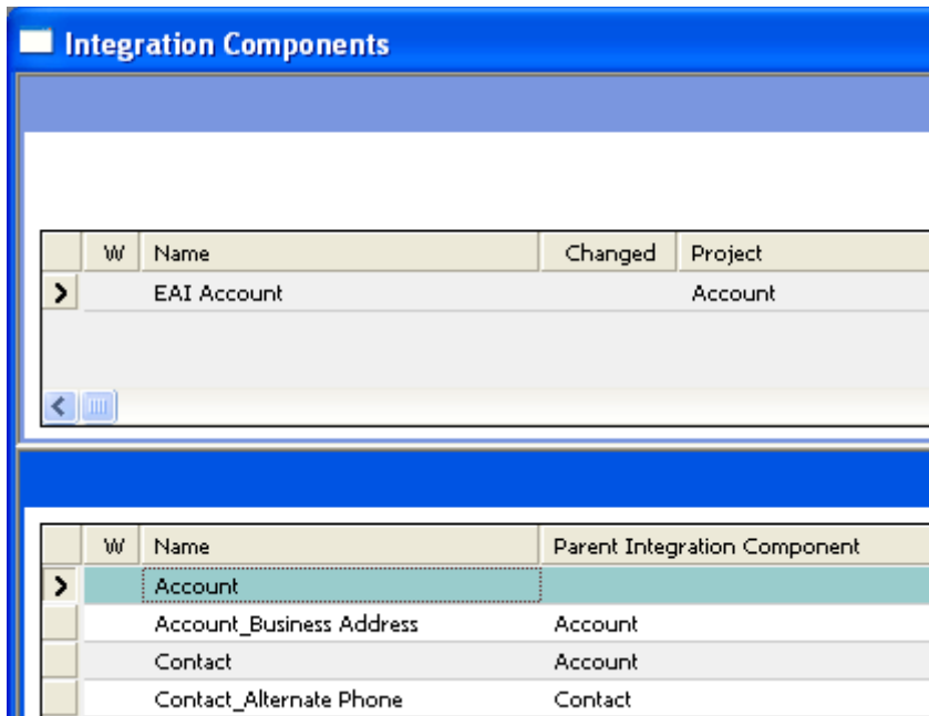
Figure 18. EAI Account Integration Object Hierarchy
